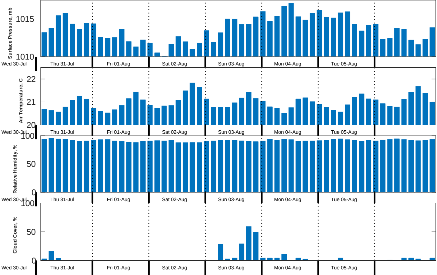
Met Forecast for CSA (ONHYM) PPL EBS - Western Sahara from 31-Jul-2025 00:00:00 to 07-Aug-2025 00:00:00
