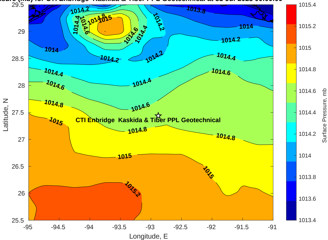
Surface Pressure (mb) for CTI Enbridge Kaskida & Tiber PPL Geotechnical at 31-Jul-2025 00:00:00
