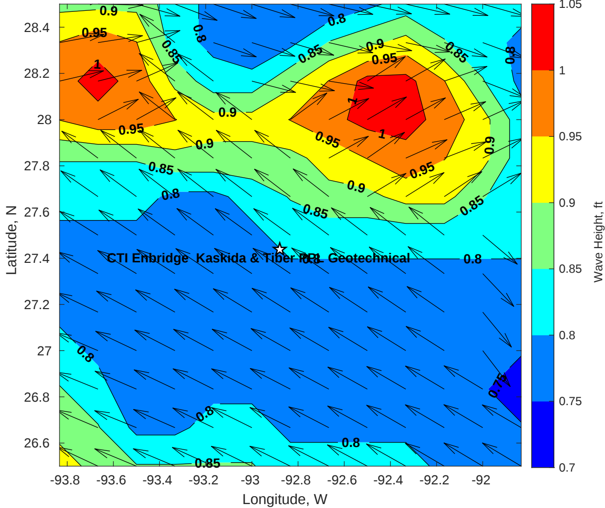
Wave Height (ft) for CTI Enbridge Kaskida & Tiber PPL Geotechnical at 31-Jul-2025 09:00:00
