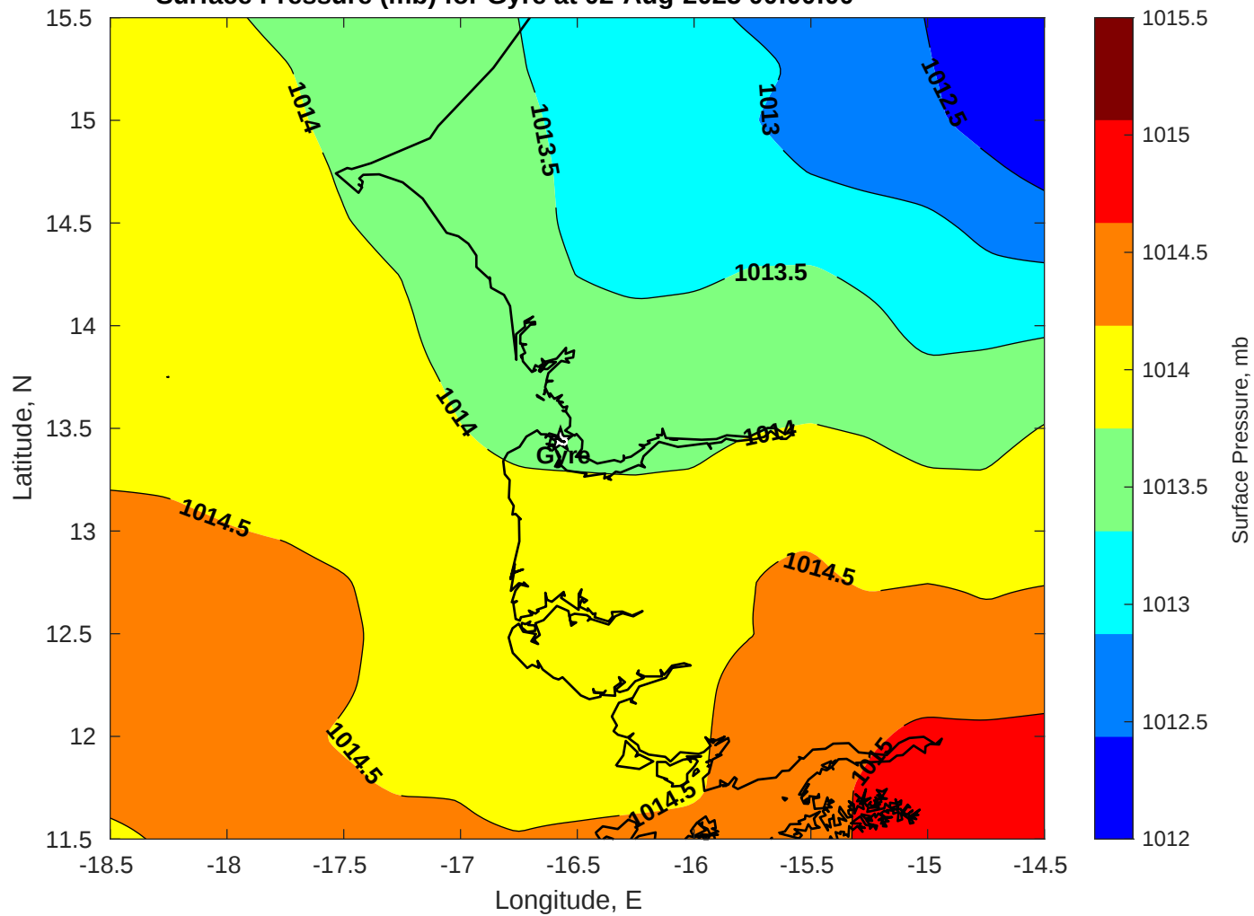
Surface Pressure (mb) for Gyre at 02-Aug-2025 00:00:00
