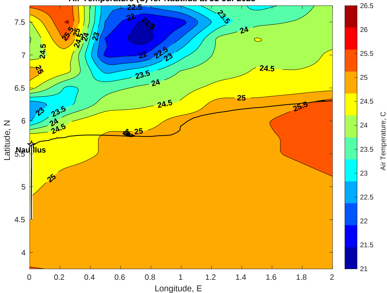
Air Temperature (C) for Nautilus at 31-Jul-2025
