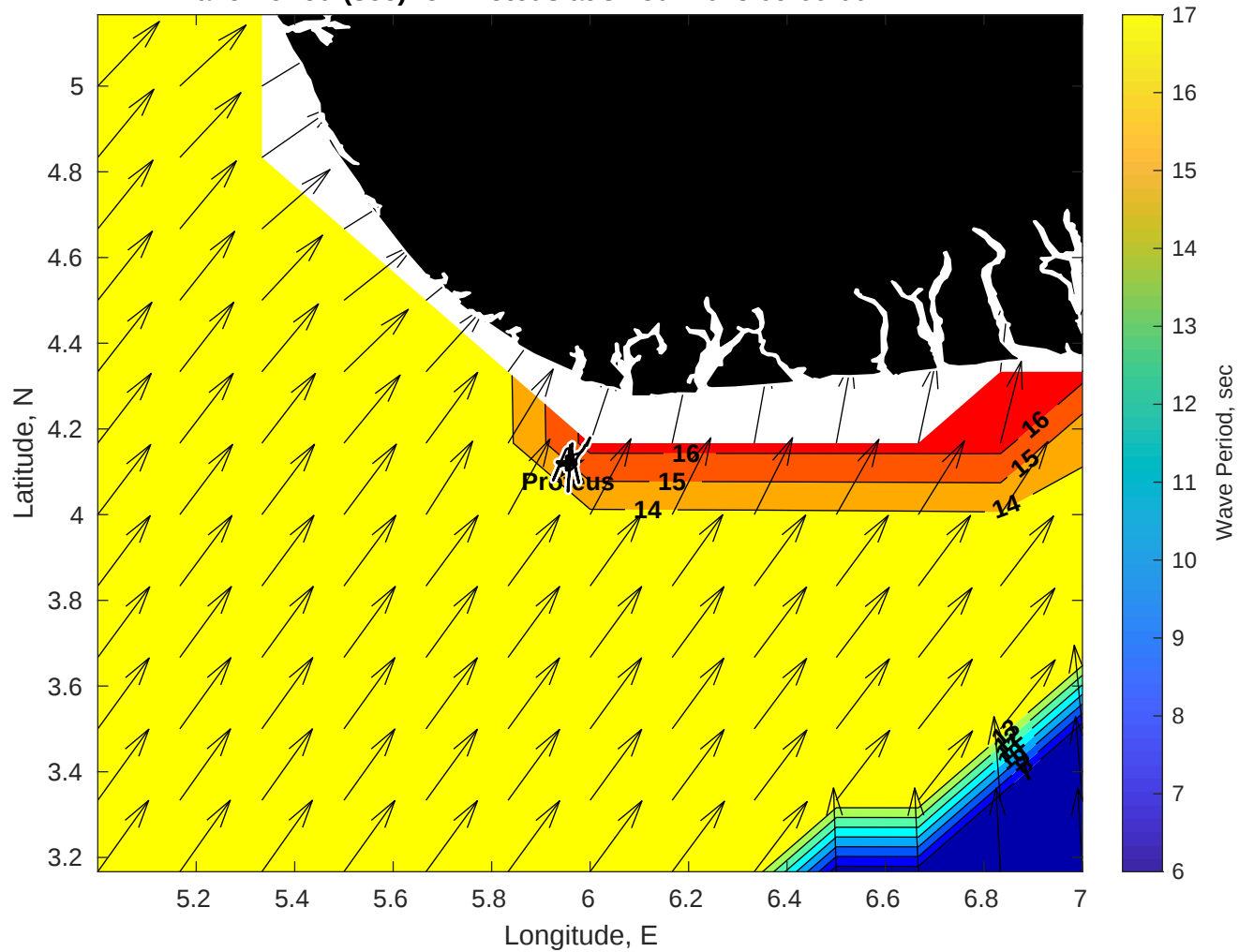
Wave Period (sec) for Proteus at 31-Jul-2025 09:00:00
