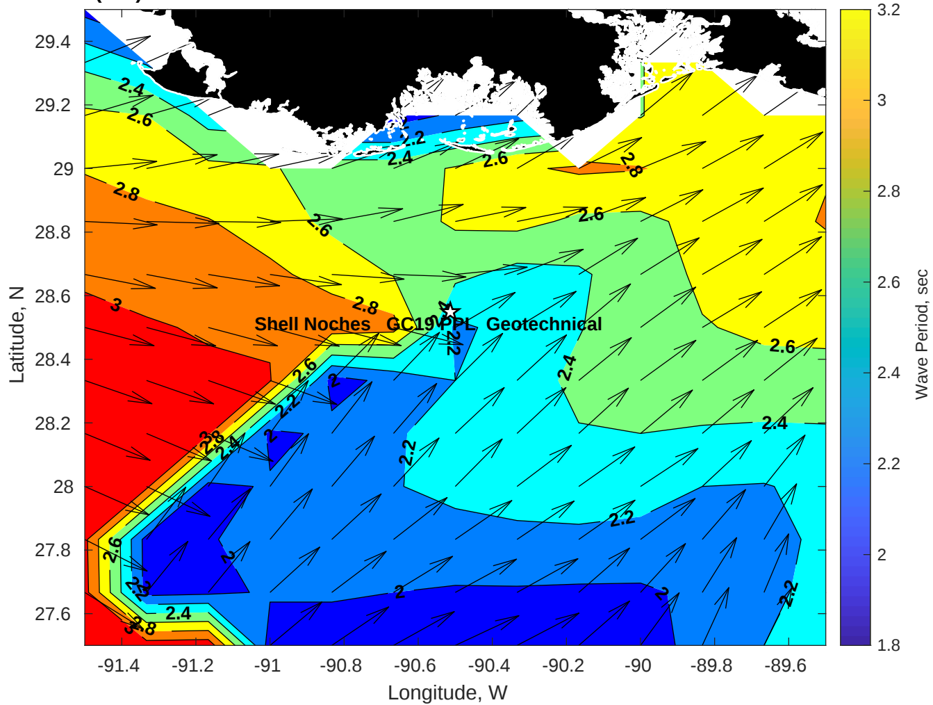
Wave Period (sec) for Shell Noches GC19 PPL Geotechnical at 31-Jul-2025 09:00:00
