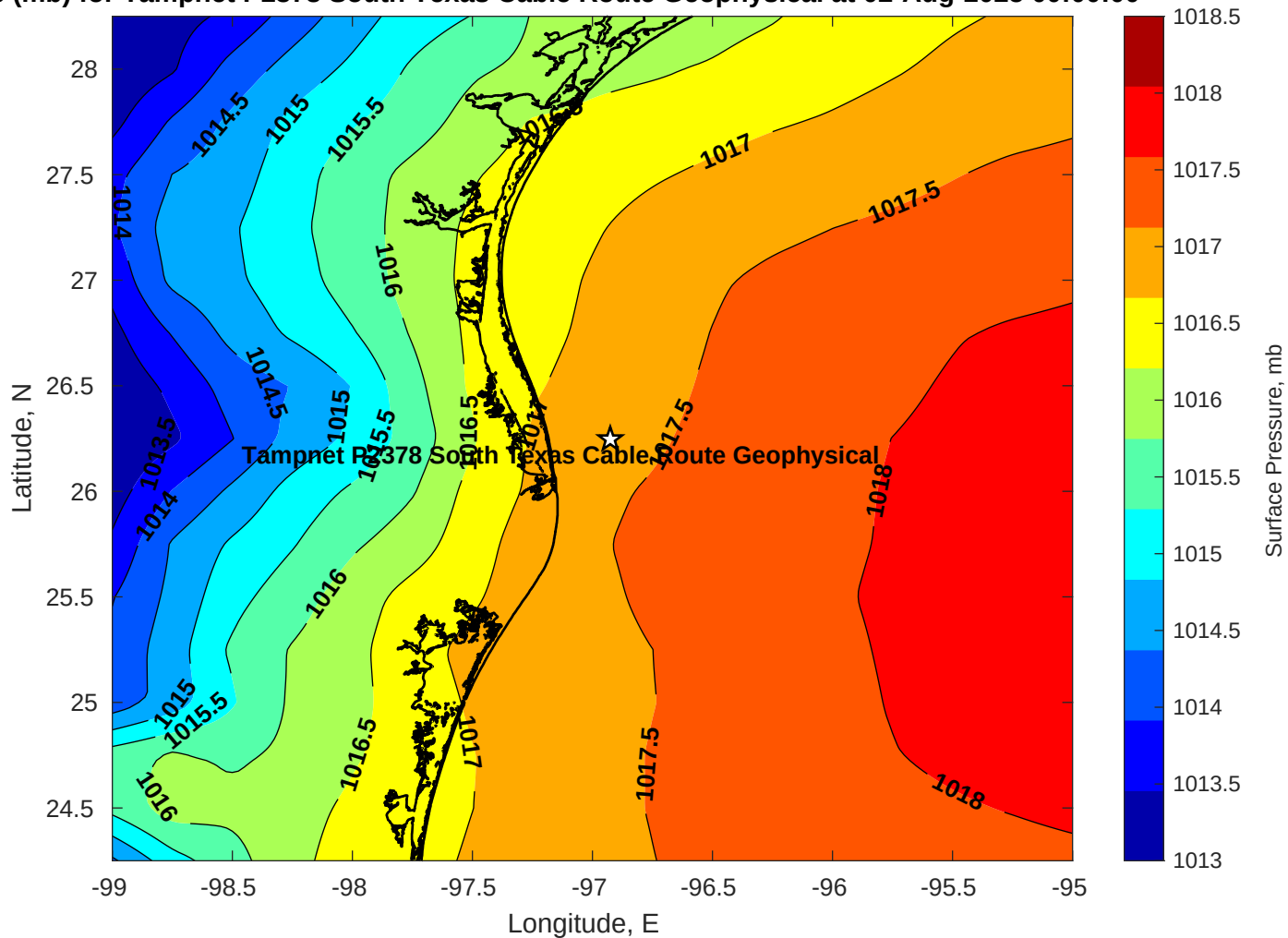
Pressure (mb) for Tampnet P2378 South Texas Cable Route Geophysical at 02-Aug-2025 00:00:00
