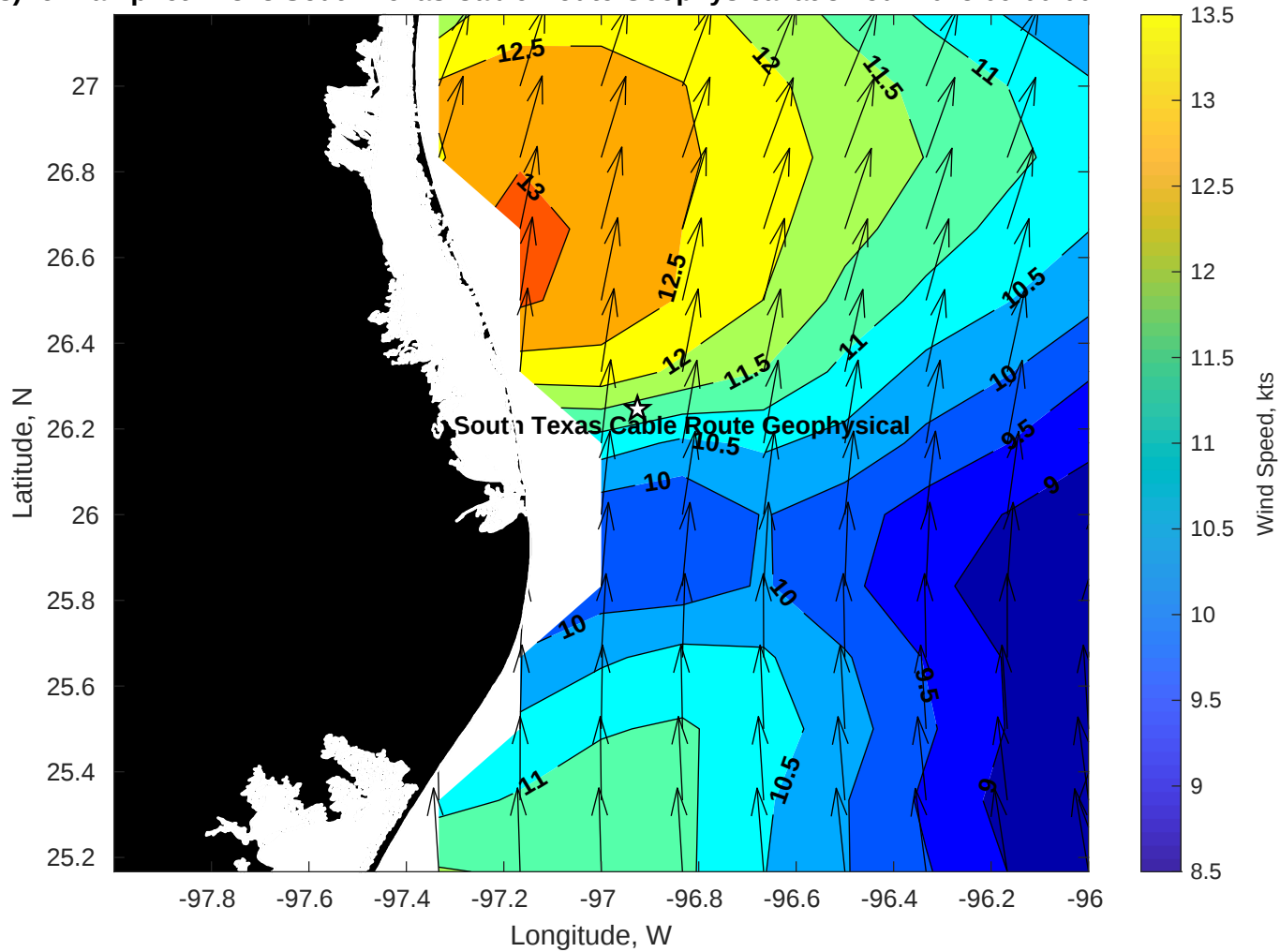
Winds (kts) for Tampnet P2378 South Texas Cable Route Geophysical at 31-Jul-2025 09:00:00
