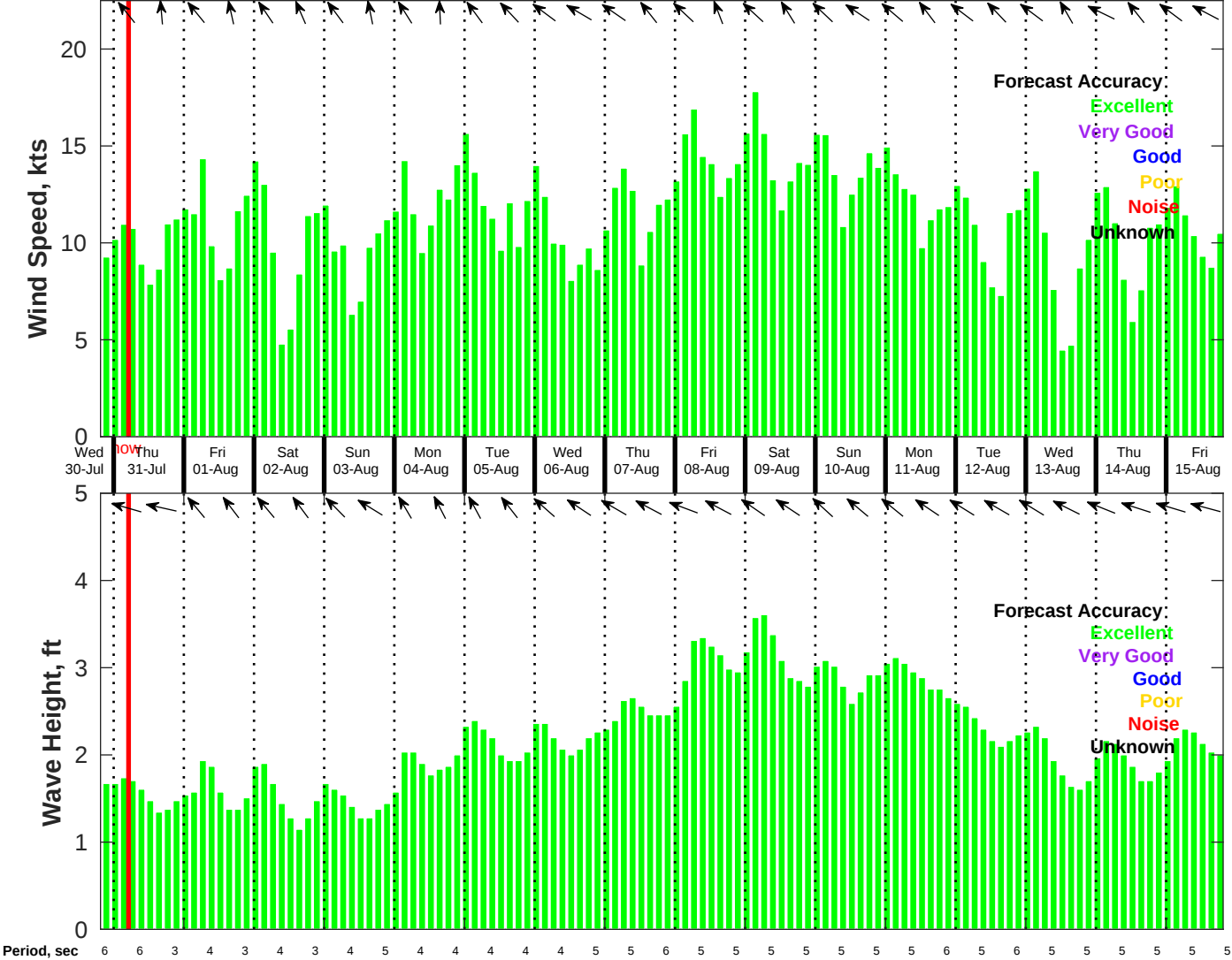
Wind & Wave Forecast for Tampnet P2378 South Texas Cable Route Geophysical from 30-Jul-2025 20:00:00 to 15-Aug-2025 20:00:00
