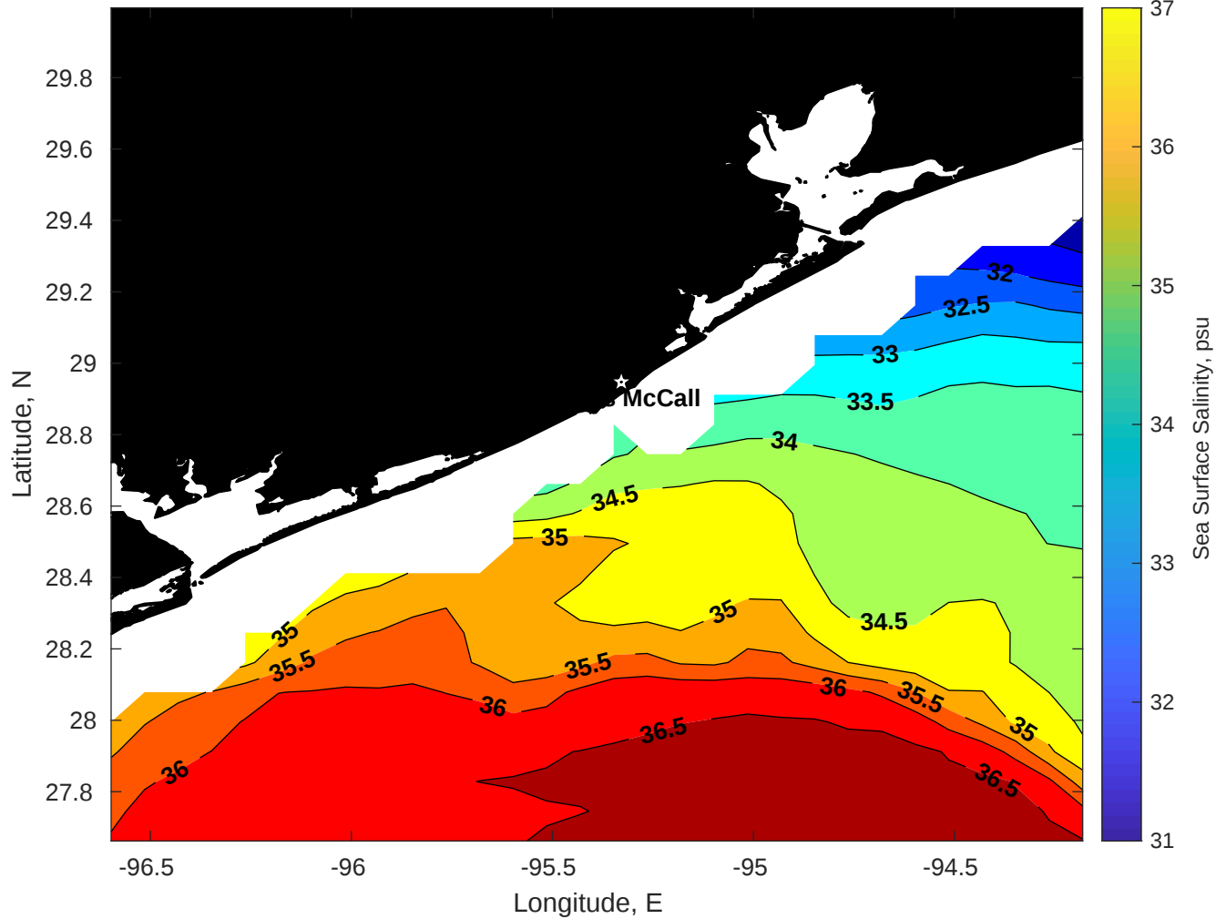
Surface Salinity for Brooks McCall at 31-Jul-2025 00:00:00
