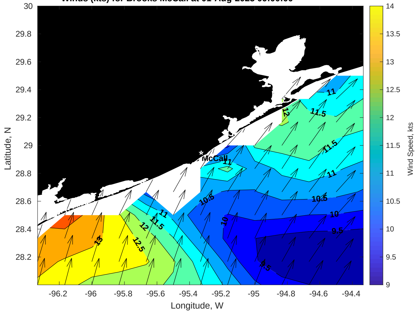
Winds (kts) for Brooks McCall at 01-Aug-2025 09:00:00
