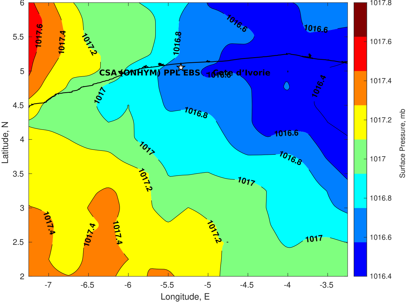
Surface Pressure (mb) for CSA (ONHYM) PPL EBS - Cote d'Ivoire at 03-Aug-2025 00:00:00
