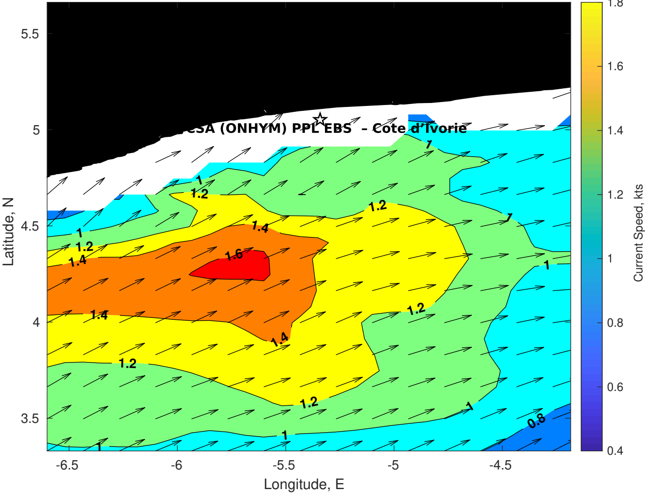
Surface Currents for CSA (ONHYM) PPL EBS - Cote d'Ivoire at 31-Jul-2025 00:00:00
