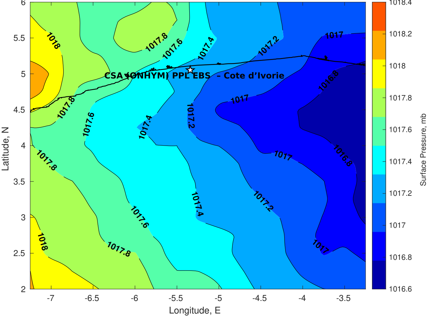
Surface Pressure (mb) for CSA (ONHYM) PPL EBS - Cote d'Ivoire at 02-Aug-2025 00:00:00
