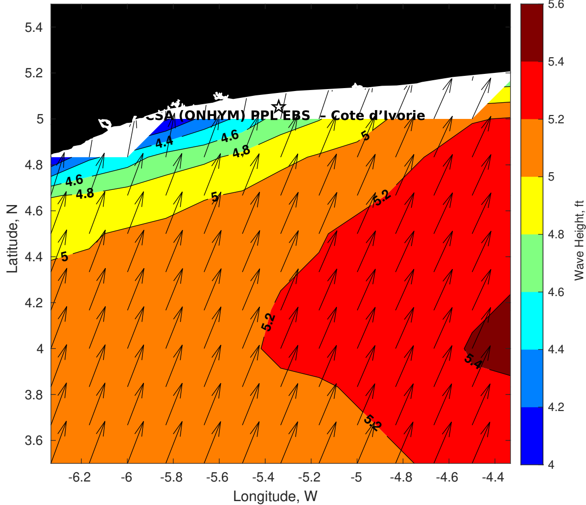
Wave Height (ft) for CSA (ONHYM) PPL EBS - Cote d'Ivoire at 01-Aug-2025 09:00:00
