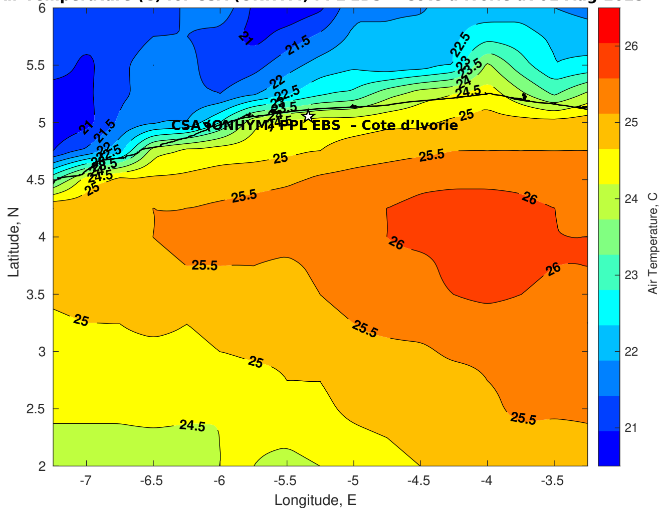
Air Temperature (C) for CSA (ONHYM) PPL EBS - Cote d'Ivoire at 01-Aug-2025
