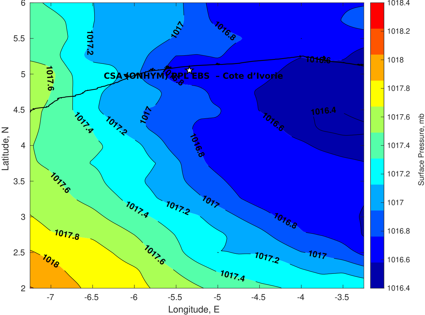
Surface Pressure (mb) for CSA (ONHYM) PPL EBS - Cote d'Ivoire at 01-Aug-2025 00:00:00
