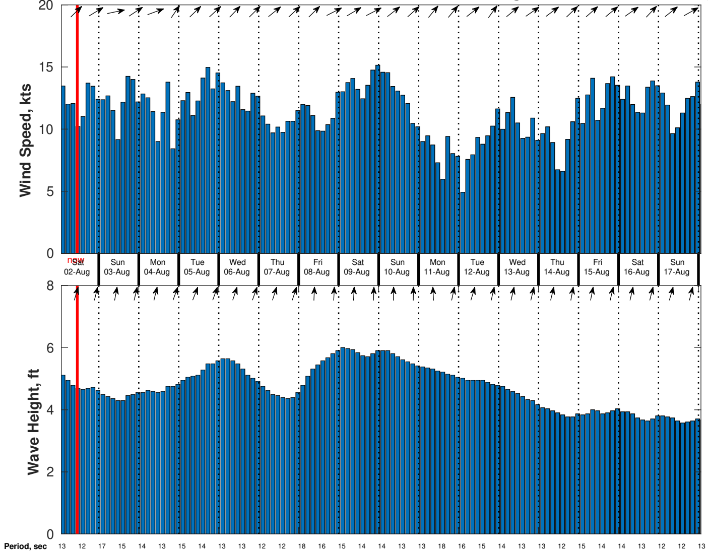
Wind & Wave Forecast for CSA (ONHYM) PPL EBS - Cote d'Ivoire from 01-Aug-2025 01:00:00 to 17-Aug-2025 01:00:00
