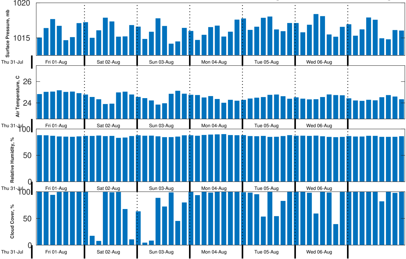
Met Forecast for CSA (ONHYM) PPL EBS - Cote d'Ivoire from 01-Aug-2025 00:00:00 to 08-Aug-2025 00:00:00
