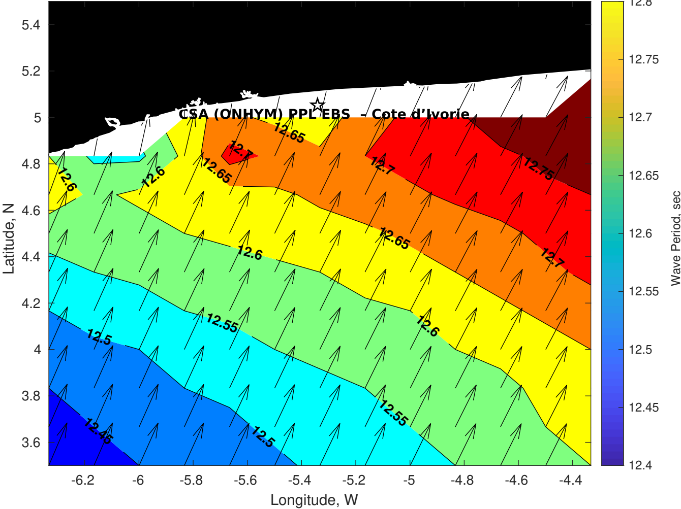
Wave Period (sec) for CSA (ONHYM) PPL EBS - Cote d'Ivoire at 01-Aug-2025 09:00:00
