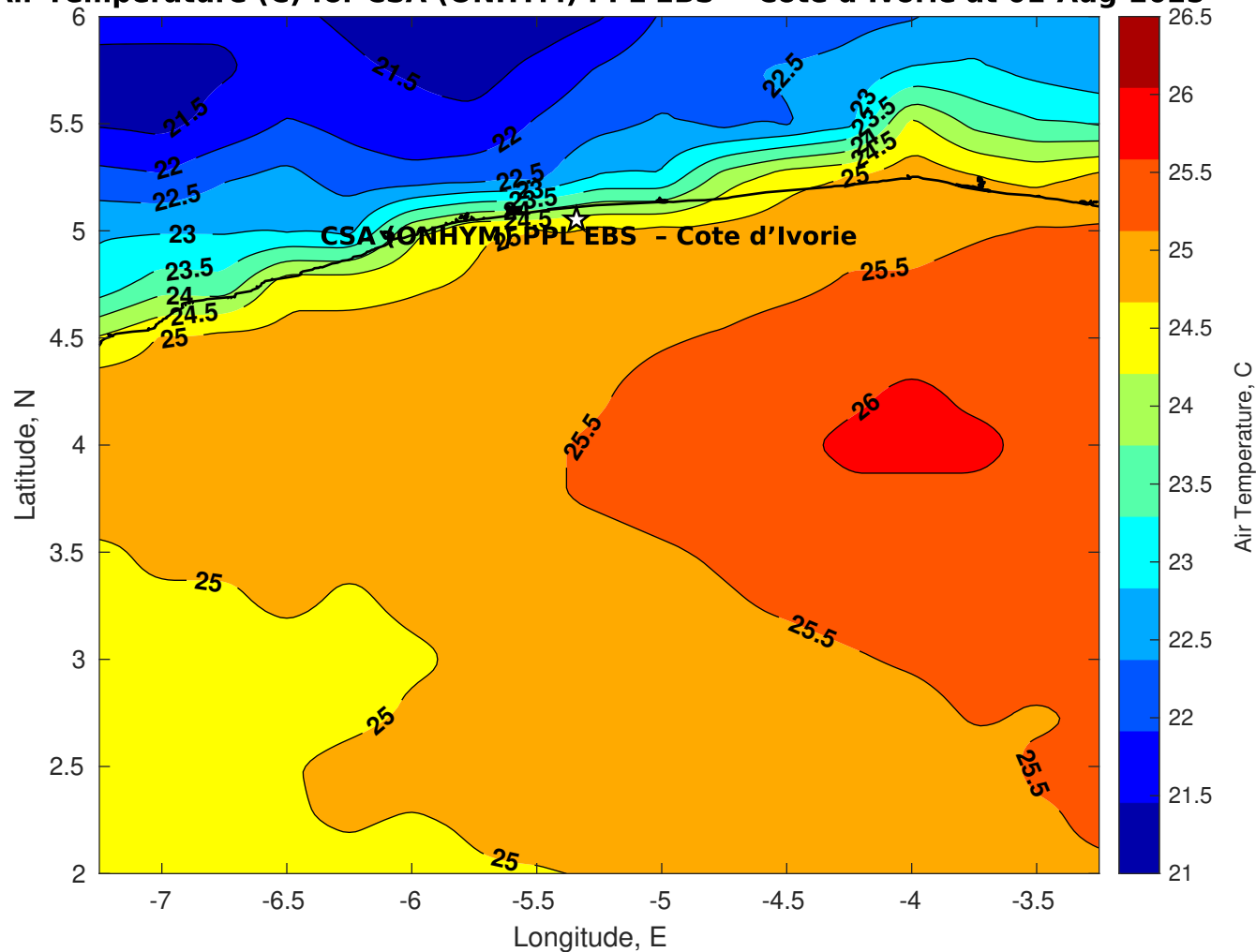
Air Temperature (C) for CSA (ONHYM) PPL EBS - Cote d'Ivoire at 01-Aug-2025
