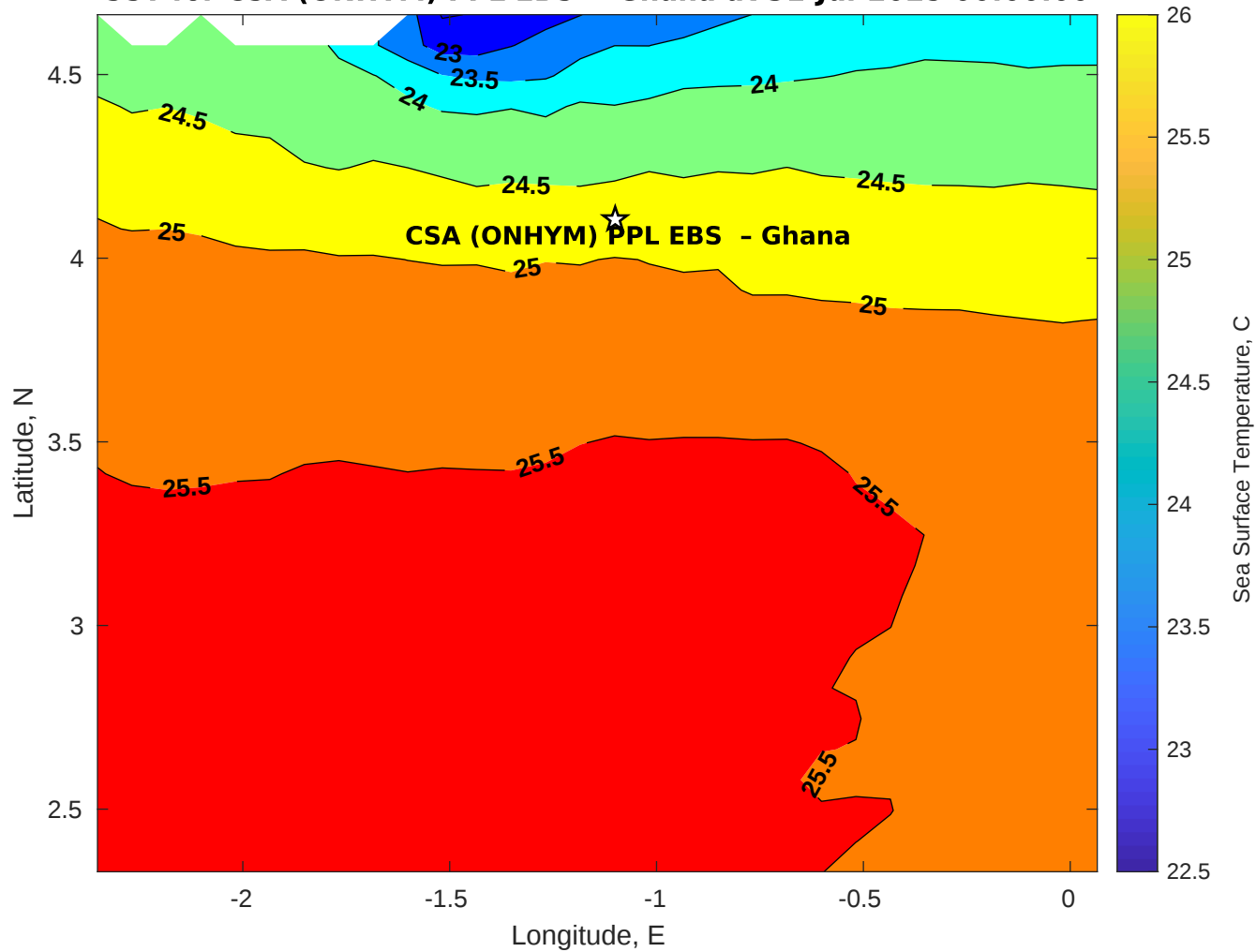
SST for CSA (ONHYM) PPL EBS - Ghana at 31-Jul-2025 00:00:00
