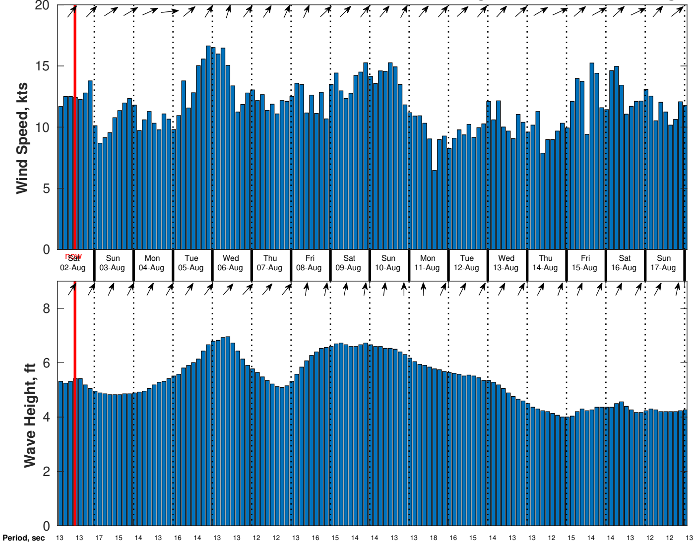
Wind & Wave Forecast for CSA (ONHYM) PPL EBS - Ghana from 01-Aug-2025 02:00:00 to 17-Aug-2025 02:00:00
