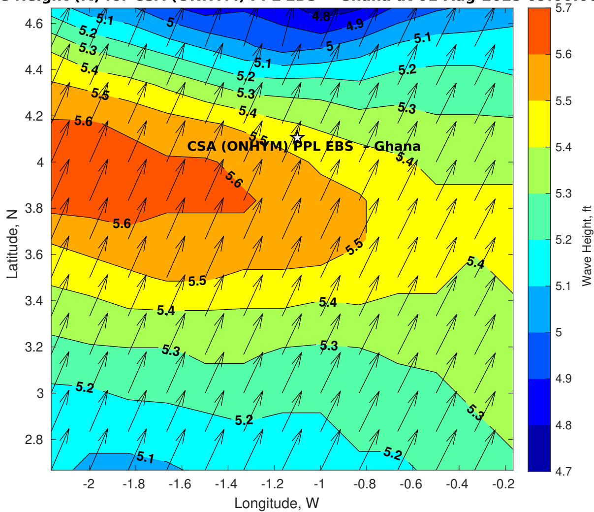
Wave Height (ft) for CSA (ONHYM) PPL EBS - Ghana at 01-Aug-2025 09:00:00
