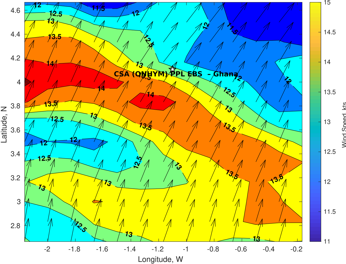
Winds (kts) for CSA (ONHYM) PPL EBS - Ghana at 01-Aug-2025 09:00:00
