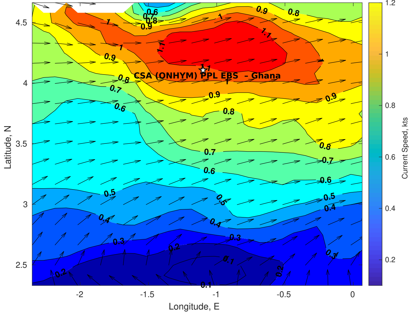
Surface Currents for CSA (ONHYM) PPL EBS - Ghana at 31-Jul-2025 00:00:00
