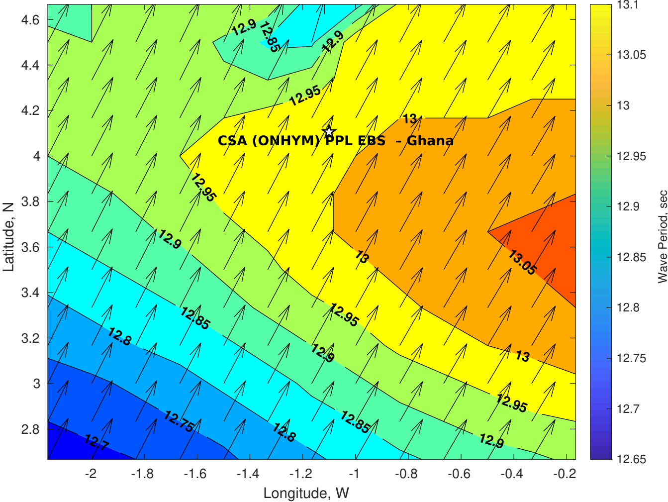
Wave Period (sec) for CSA (ONHYM) PPL EBS - Ghana at 01-Aug-2025 09:00:00
