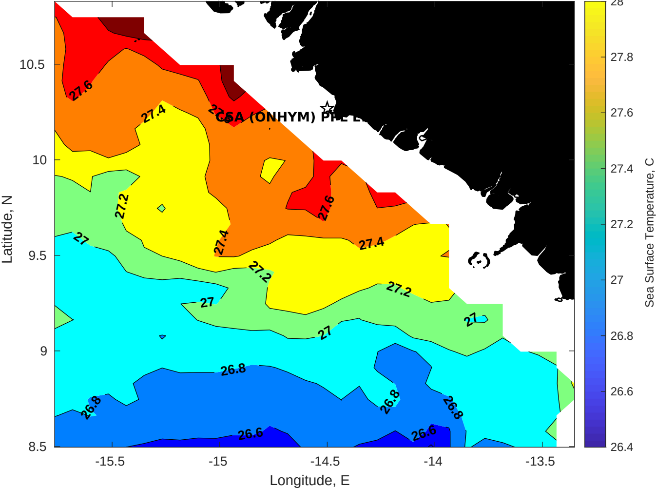
SST for CSA (ONHYM) PPL EBS - Guinea at 31-Jul-2025 00:00:00
