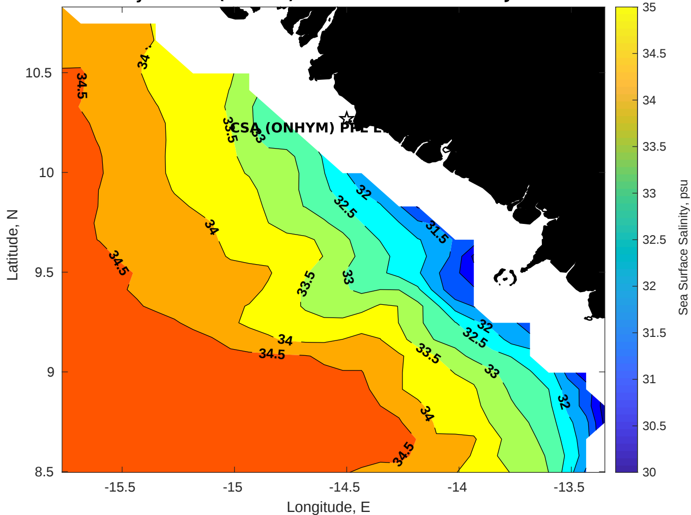
Surface Salinity for CSA (ONHYM) PPL EBS - Guinea at 31-Jul-2025 00:00:00
