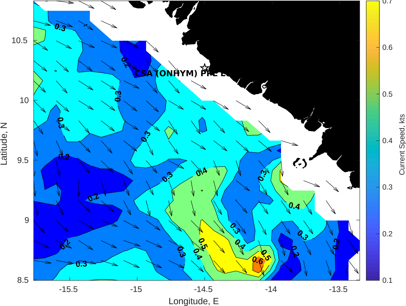
Surface Currents for CSA (ONHYM) PPL EBS - Guinea at 31-Jul-2025 00:00:00
