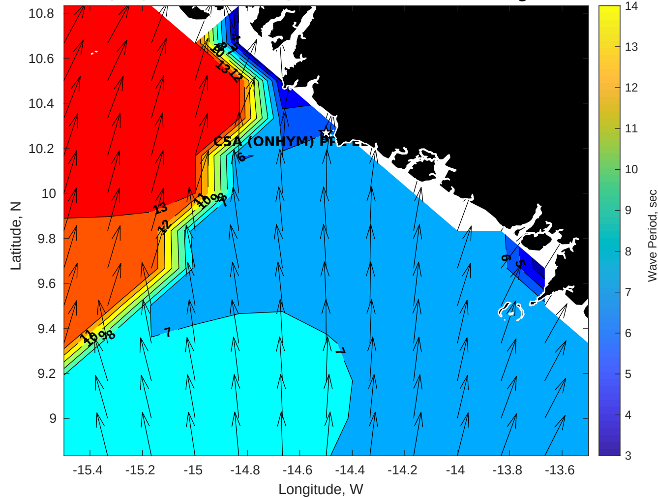
Wave Period (sec) for CSA (ONHYM) PPL EBS - Guinea at 01-Aug-2025 09:00:00
