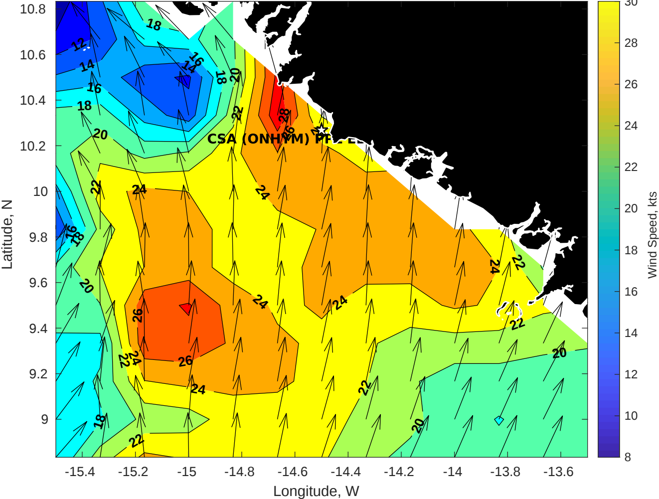
Winds (kts) for CSA (ONHYM) PPL EBS - Guinea at 01-Aug-2025 09:00:00
