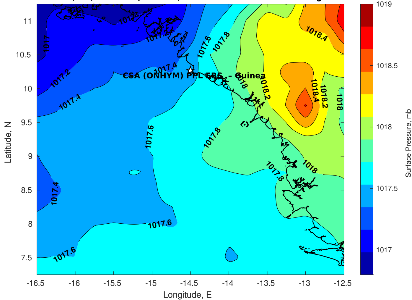
Surface Pressure (mb) for CSA (ONHYM) PPL EBS - Guinea at 03-Aug-2025 00:00:00
