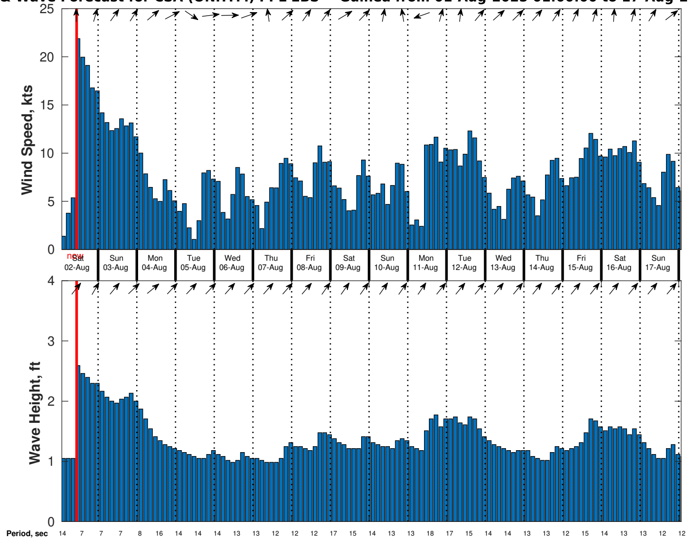
Wind & Wave Forecast for CSA (ONHYM) PPL EBS - Guinea from 01-Aug-2025 01:00:00 to 17-Aug-2025 01:00:00
