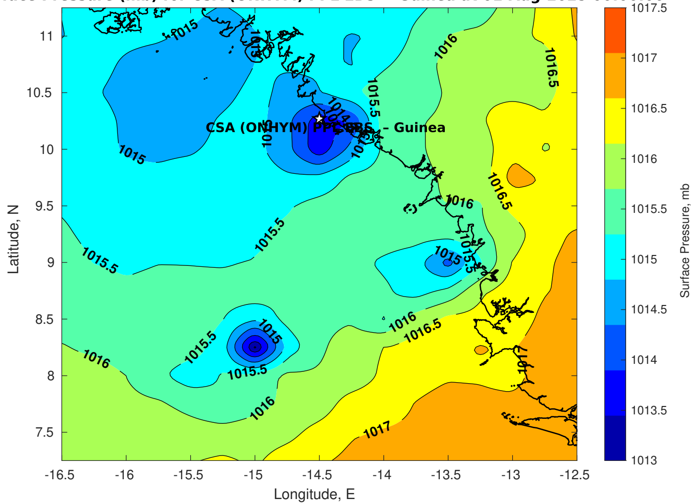
Surface Pressure (mb) for CSA (ONHYM) PPL EBS - Guinea at 01-Aug-2025 00:00:00
