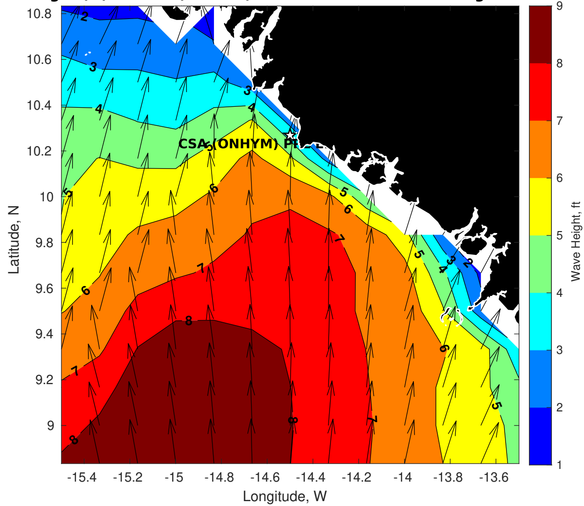
Wave Height (ft) for CSA (ONHYM) PPL EBS - Guinea at 01-Aug-2025 09:00:00
