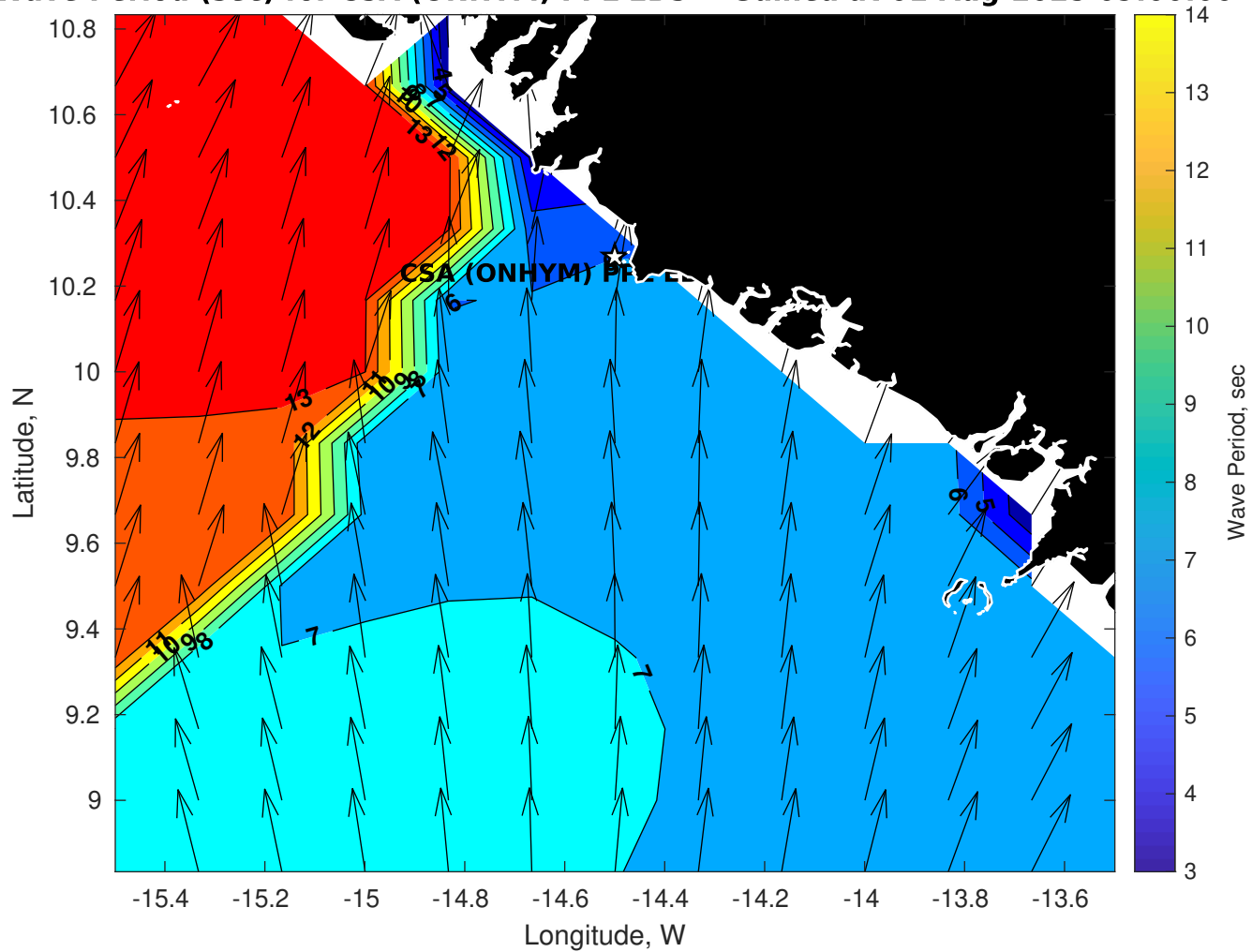
Wave Period (sec) for CSA (ONHYM) PPL EBS - Guinea at 01-Aug-2025 09:00:00
