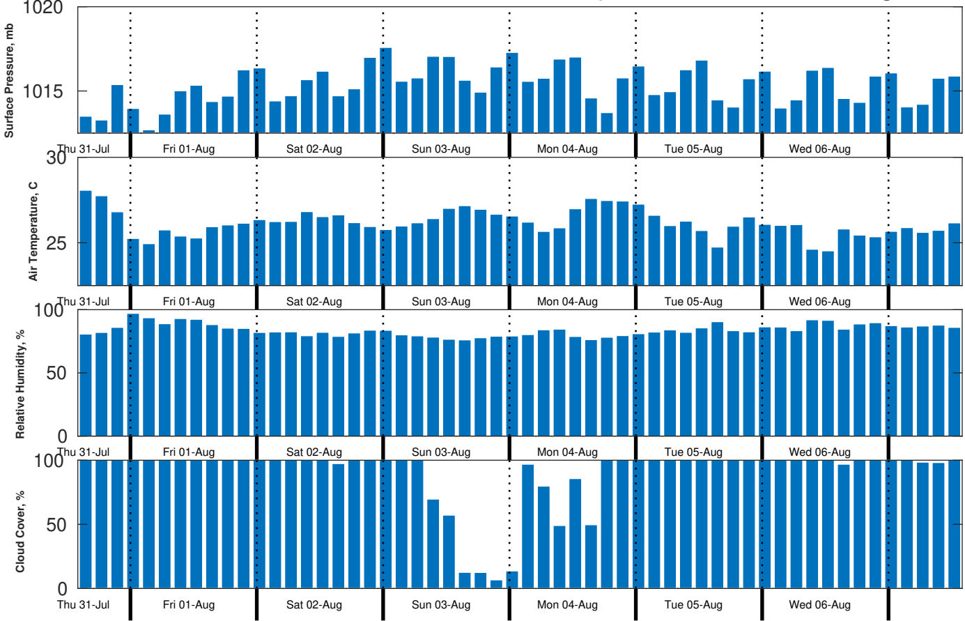
Met Forecast for CSA (ONHYM) PPL EBS - Guinea from 31-Jul-2025 12:00:00 to 07-Aug-2025 12:00:00
