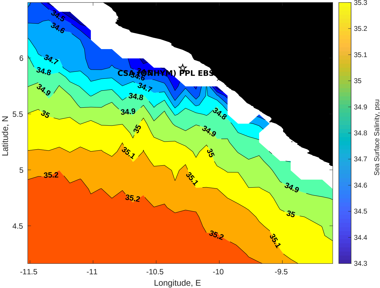
Surface Salinity for CSA (ONHYM) PPL EBS - Liberia at 31-Jul-2025 00:00:00
