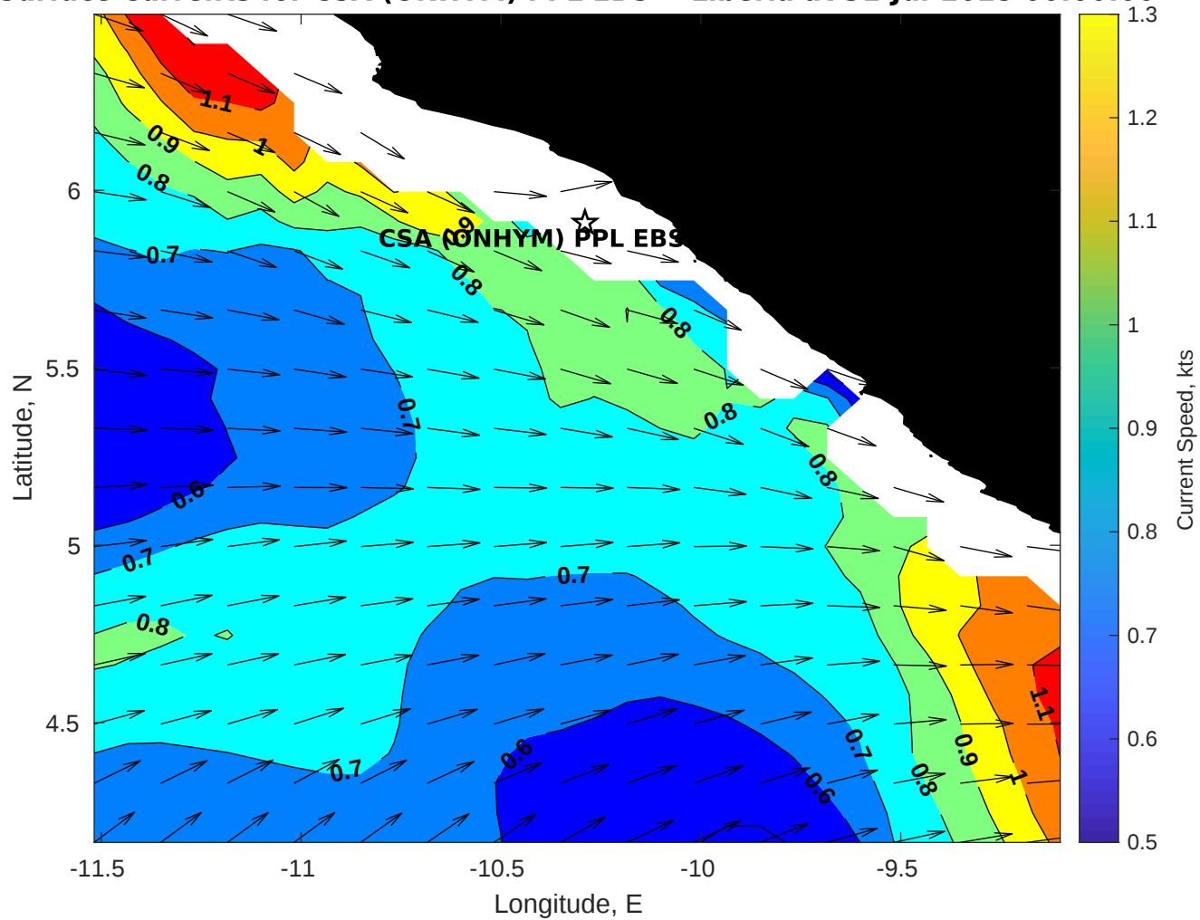
Surface Currents for CSA (ONHYM) PPL EBS - Liberia at 31-Jul-2025 00:00:00
