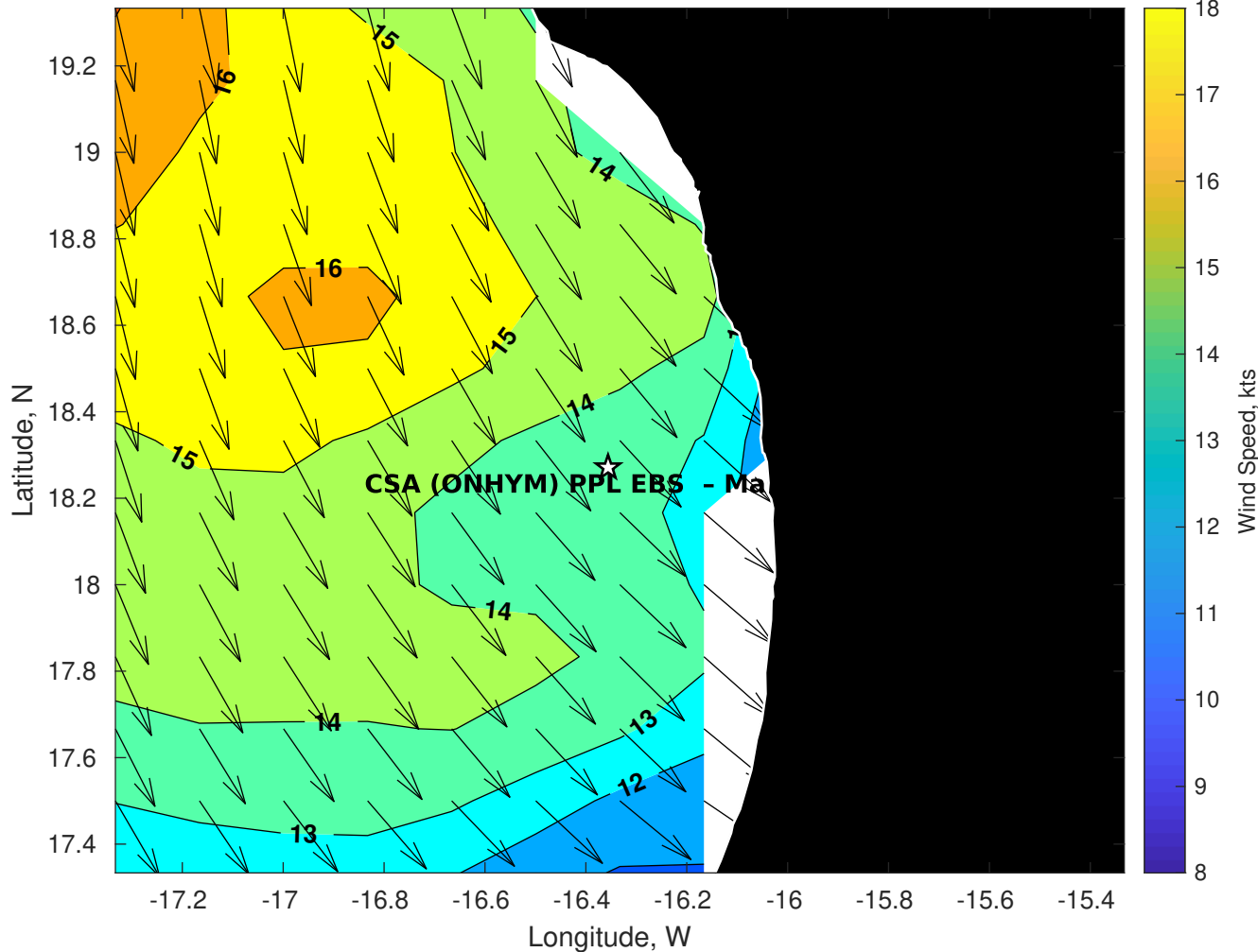
Winds (kts) for CSA (ONHYM) PPL EBS - Mauritania at 01-Aug-2025 09:00:00
