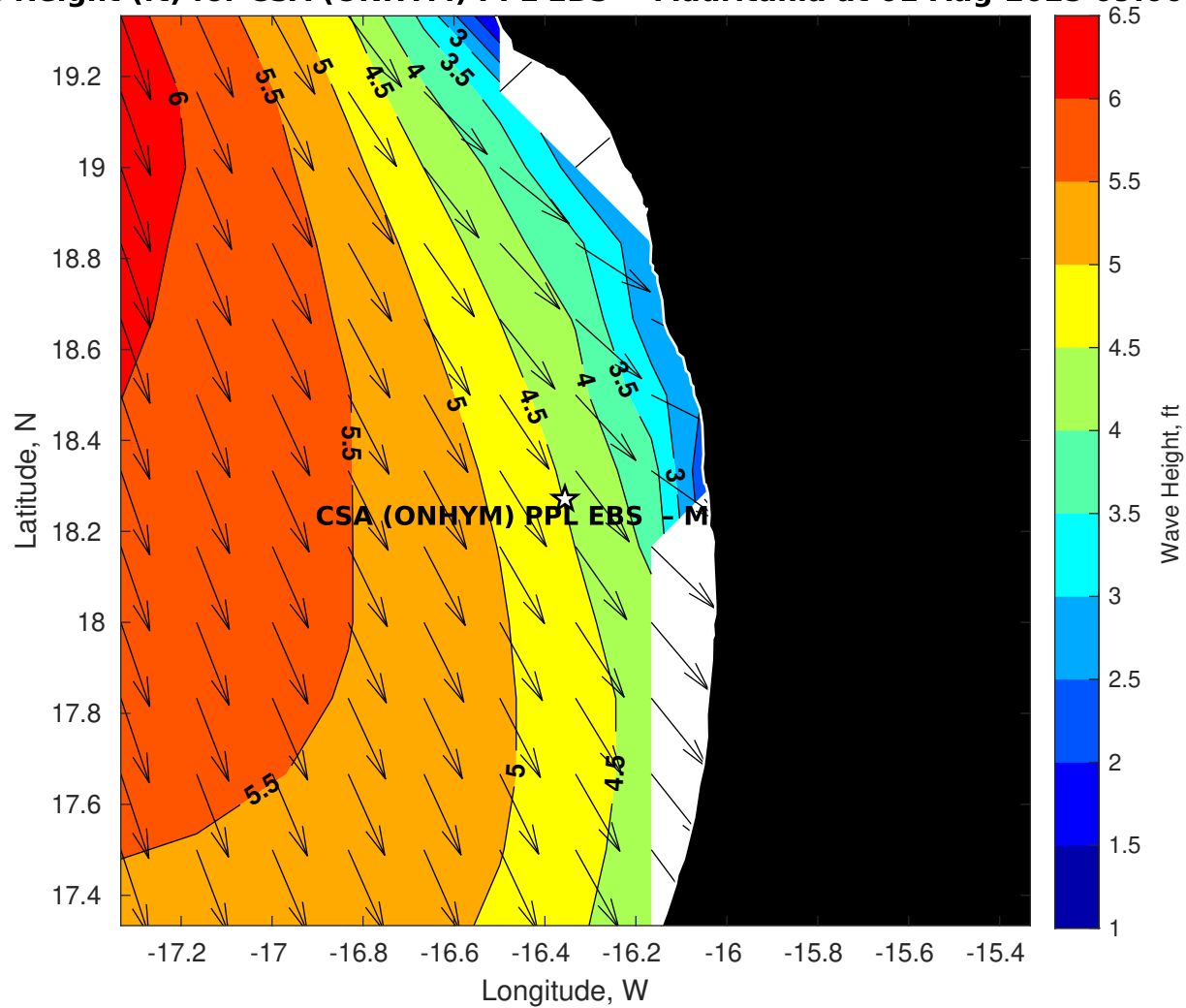
Wave Height (ft) for CSA (ONHYM) PPL EBS - Mauritania at 01-Aug-2025 09:00:00
