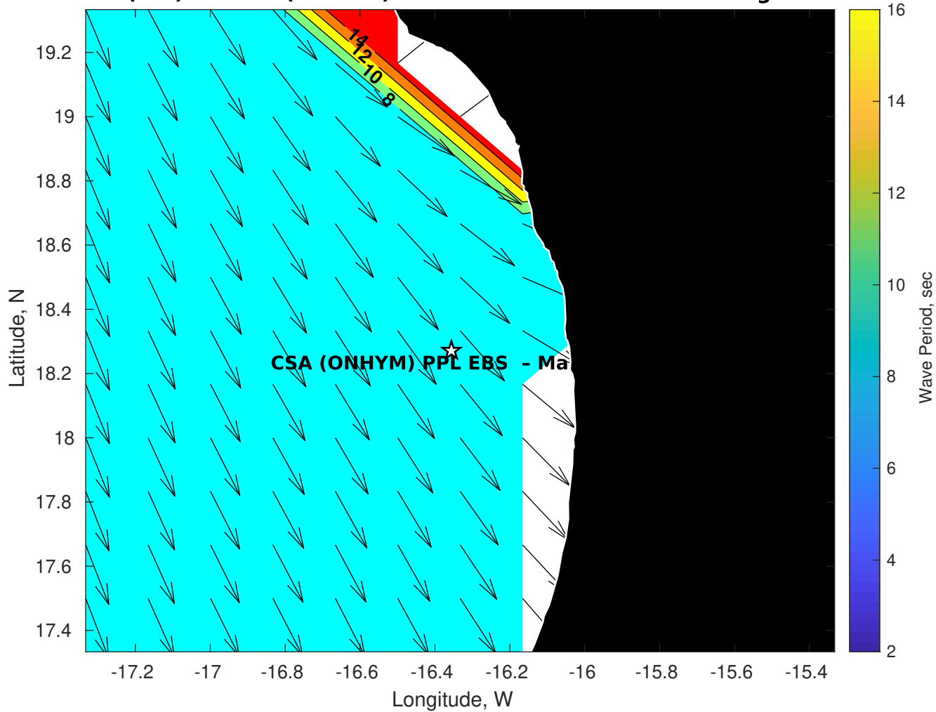
Wave Period (sec) for CSA (ONHYM) PPL EBS - Mauritania at 01-Aug-2025 09:00:00
