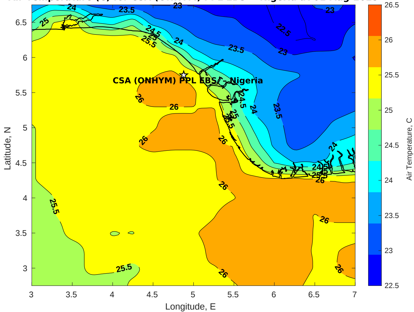
Air Temperature (C) for CSA (ONHYM) PPL EBS - Nigeria at 01-Aug-2025
