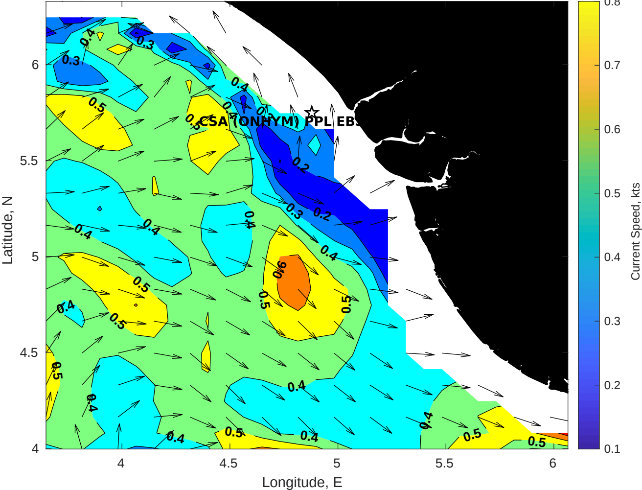
Surface Currents for CSA (ONHYM) PPL EBS - Nigeria at 31-Jul-2025 00:00:00
