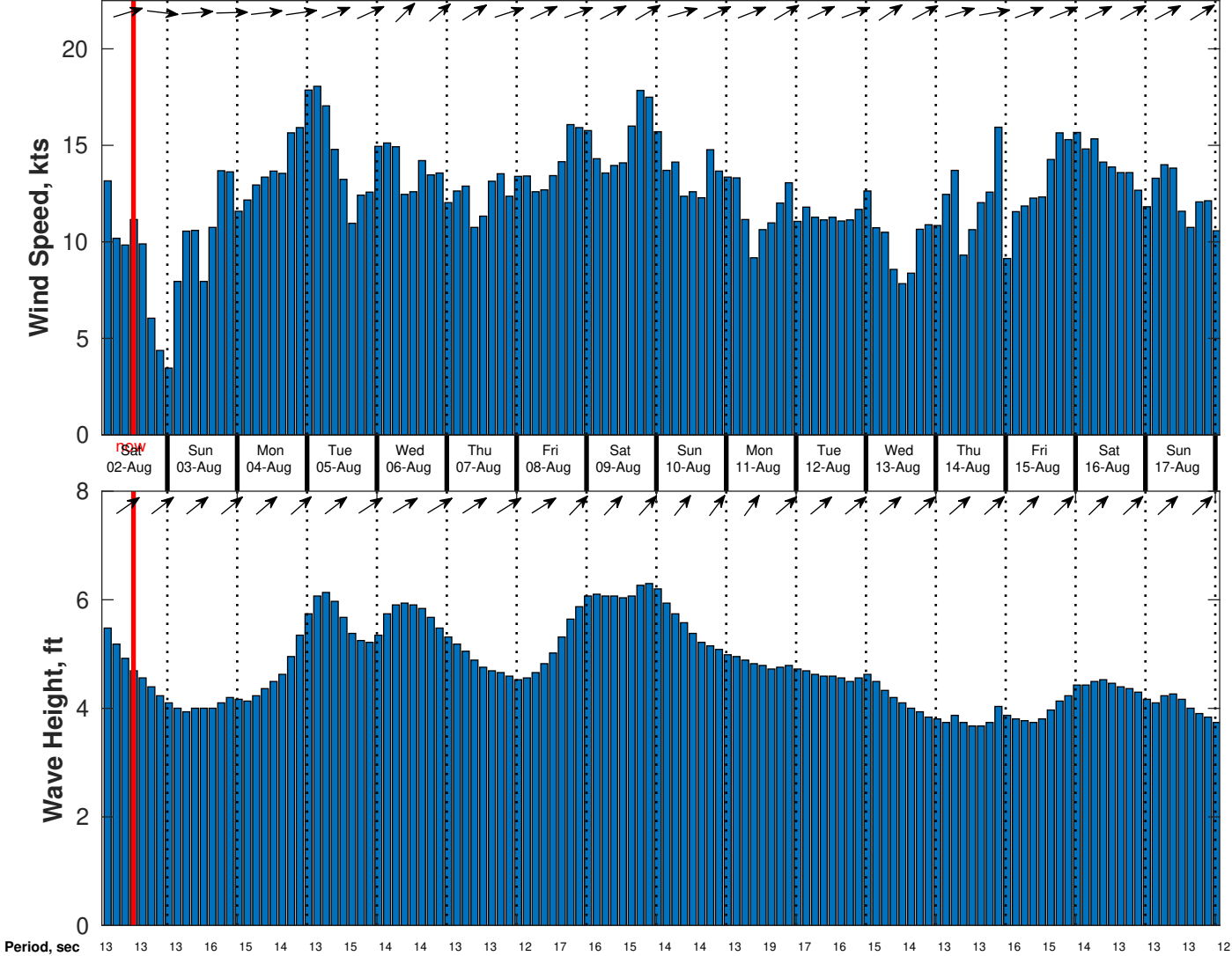
Wind & Wave Forecast for CSA (ONHYM) PPL EBS - Nigeria from 01-Aug-2025 02:00:00 to 17-Aug-2025 02:00:00
