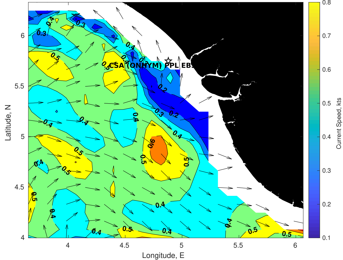
Surface Currents for CSA (ONHYM) PPL EBS - Nigeria at 31-Jul-2025 00:00:00
