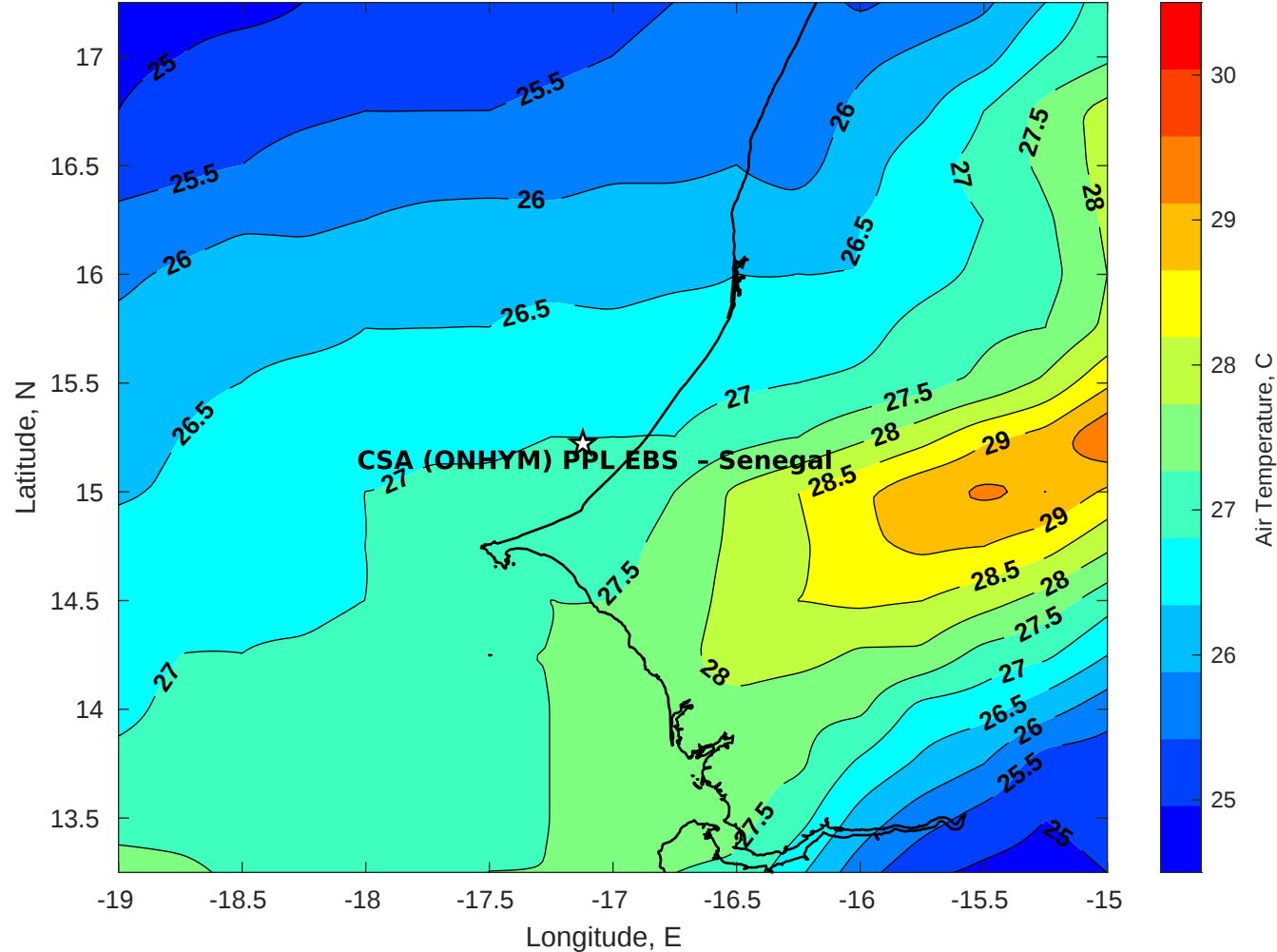
Air Temperature (C) for CSA (ONHYM) PPL EBS - Senegal at 01-Aug-2025
