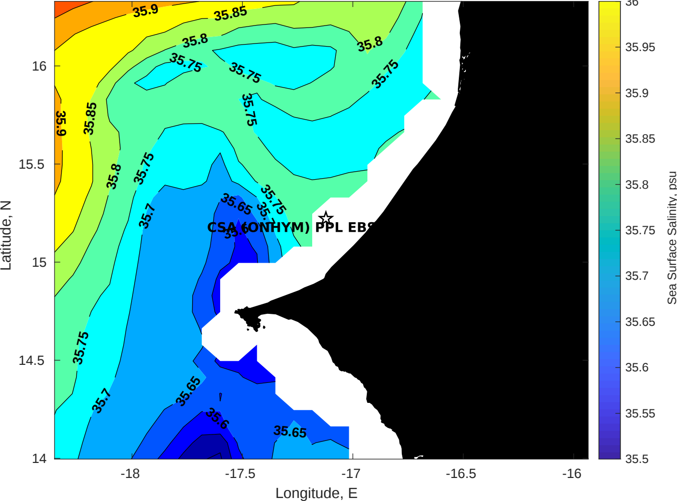
Surface Salinity for CSA (ONHYM) PPL EBS - Senegal at 31-Jul-2025 00:00:00
