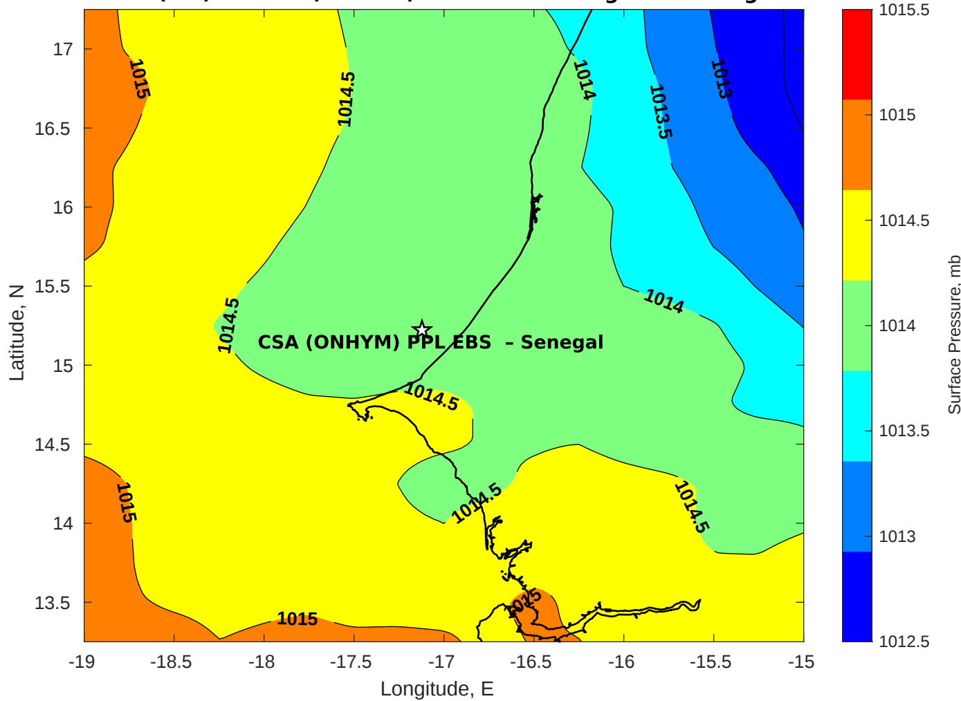
Surface Pressure (mb) for CSA (ONHYM) PPL EBS - Senegal at 01-Aug-2025 00:00:00
