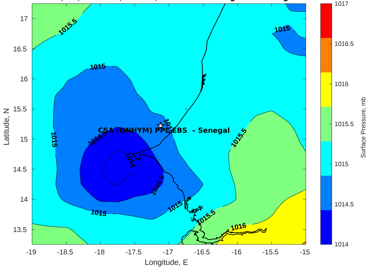
Surface Pressure (mb) for CSA (ONHYM) PPL EBS - Senegal at 03-Aug-2025 00:00:00
