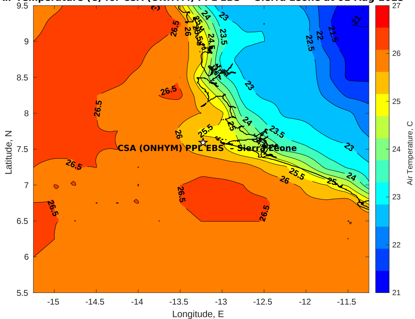
Air Temperature (C) for CSA (ONHYM) PPL EBS - Sierra Leone at 01-Aug-2025
