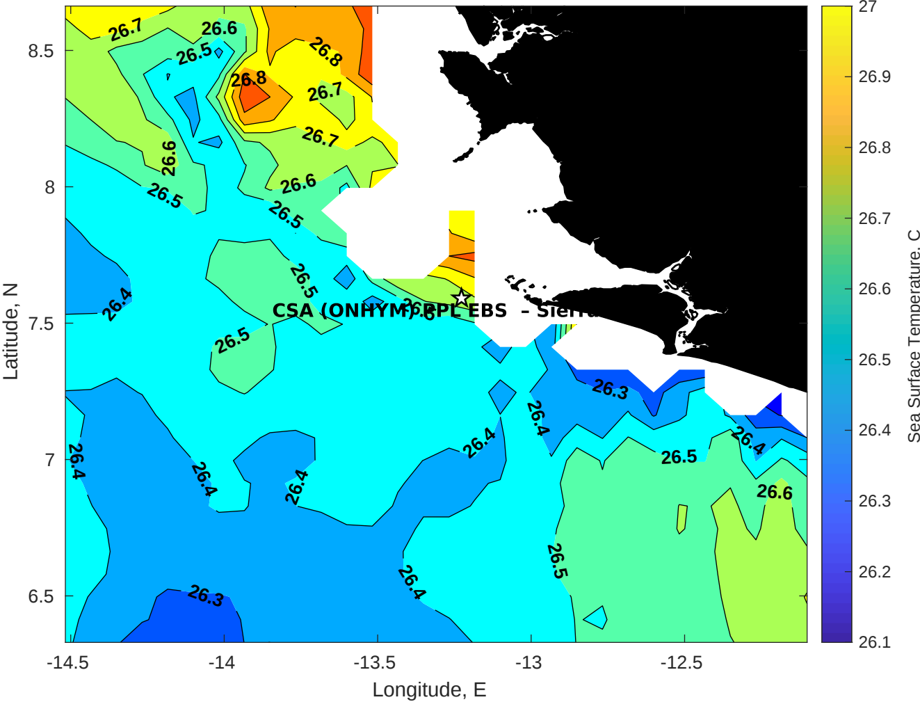
SST for CSA (ONHYM) PPL EBS - Sierra Leone at 31-Jul-2025 00:00:00
