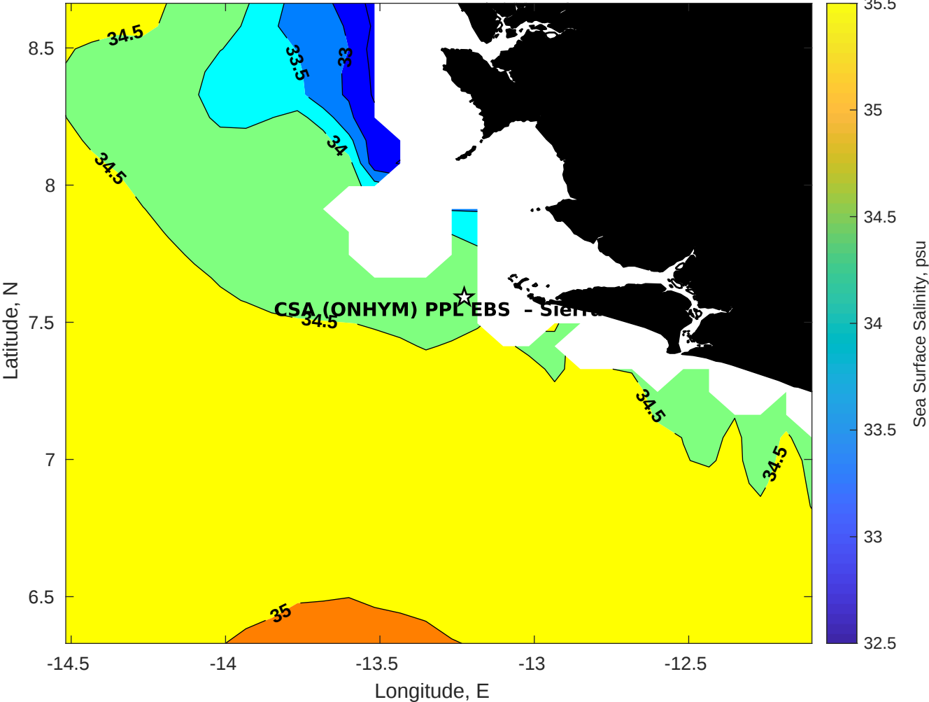
Surface Salinity for CSA (ONHYM) PPL EBS - Sierra Leone at 31-Jul-2025 00:00:00
