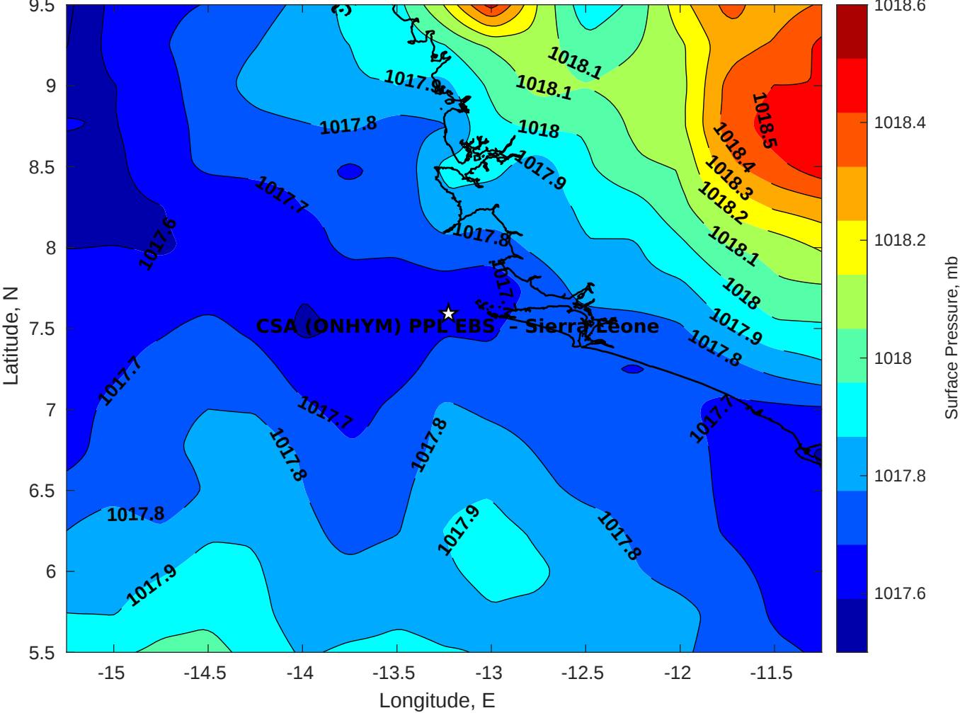
Surface Pressure (mb) for CSA (ONHYM) PPL EBS - Sierra Leone at 03-Aug-2025 00:00:00
