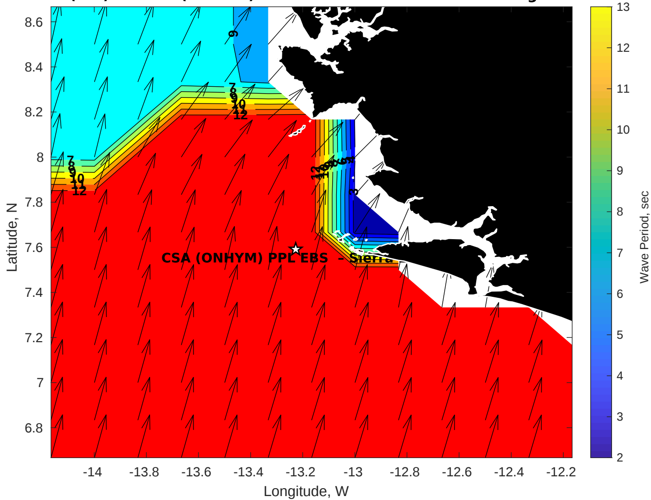
Wave Period (sec) for CSA (ONHYM) PPL EBS - Sierra Leone at 01-Aug-2025 09:00:00
