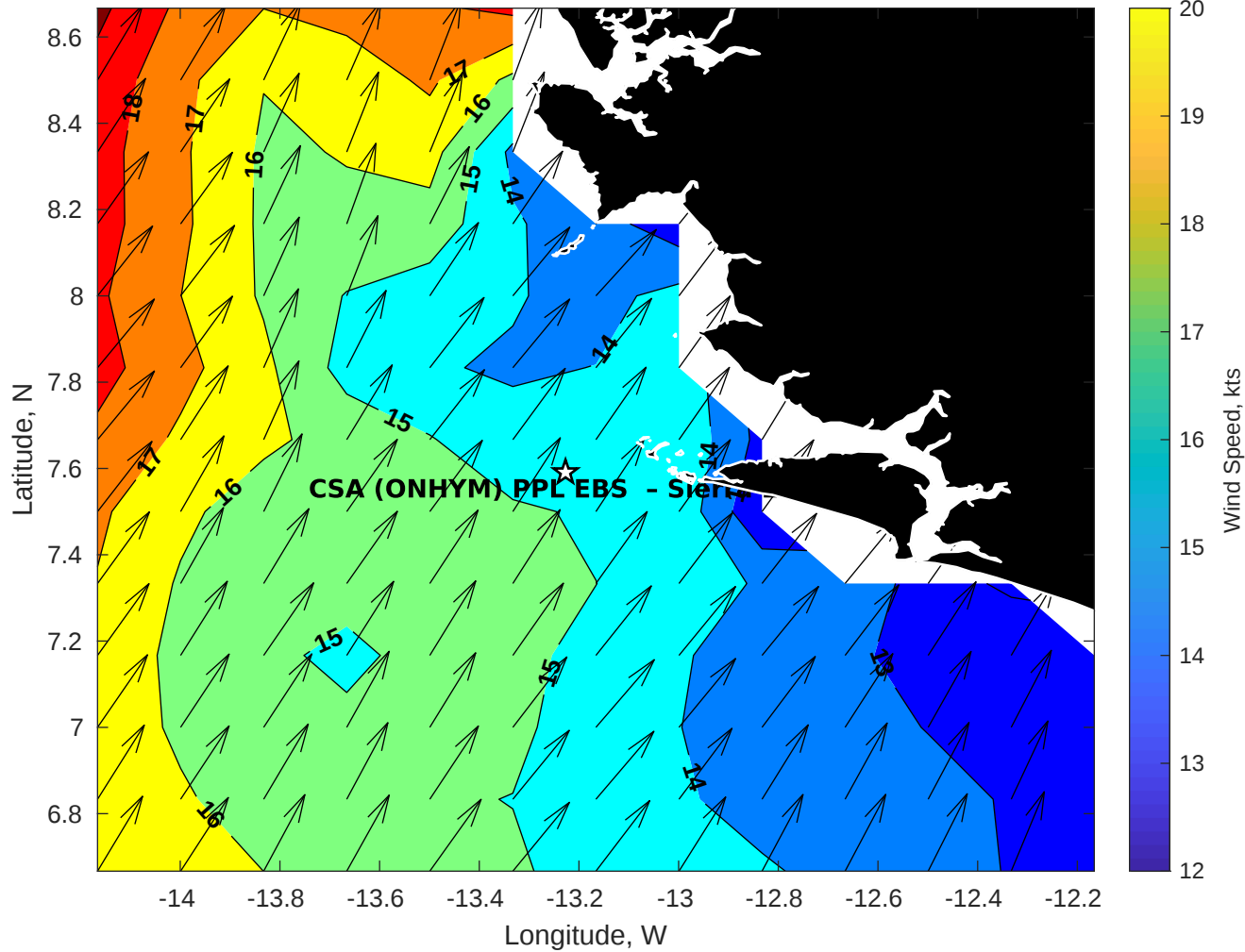
Winds (kts) for CSA (ONHYM) PPL EBS - Sierra Leone at 01-Aug-2025 09:00:00
