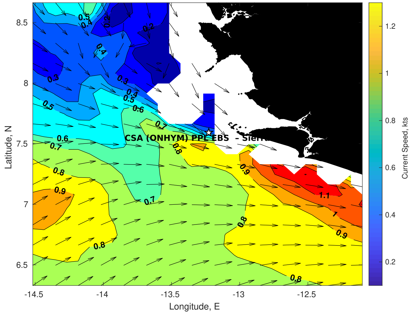
Surface Currents for CSA (ONHYM) PPL EBS - Sierra Leone at 31-Jul-2025 00:00:00
