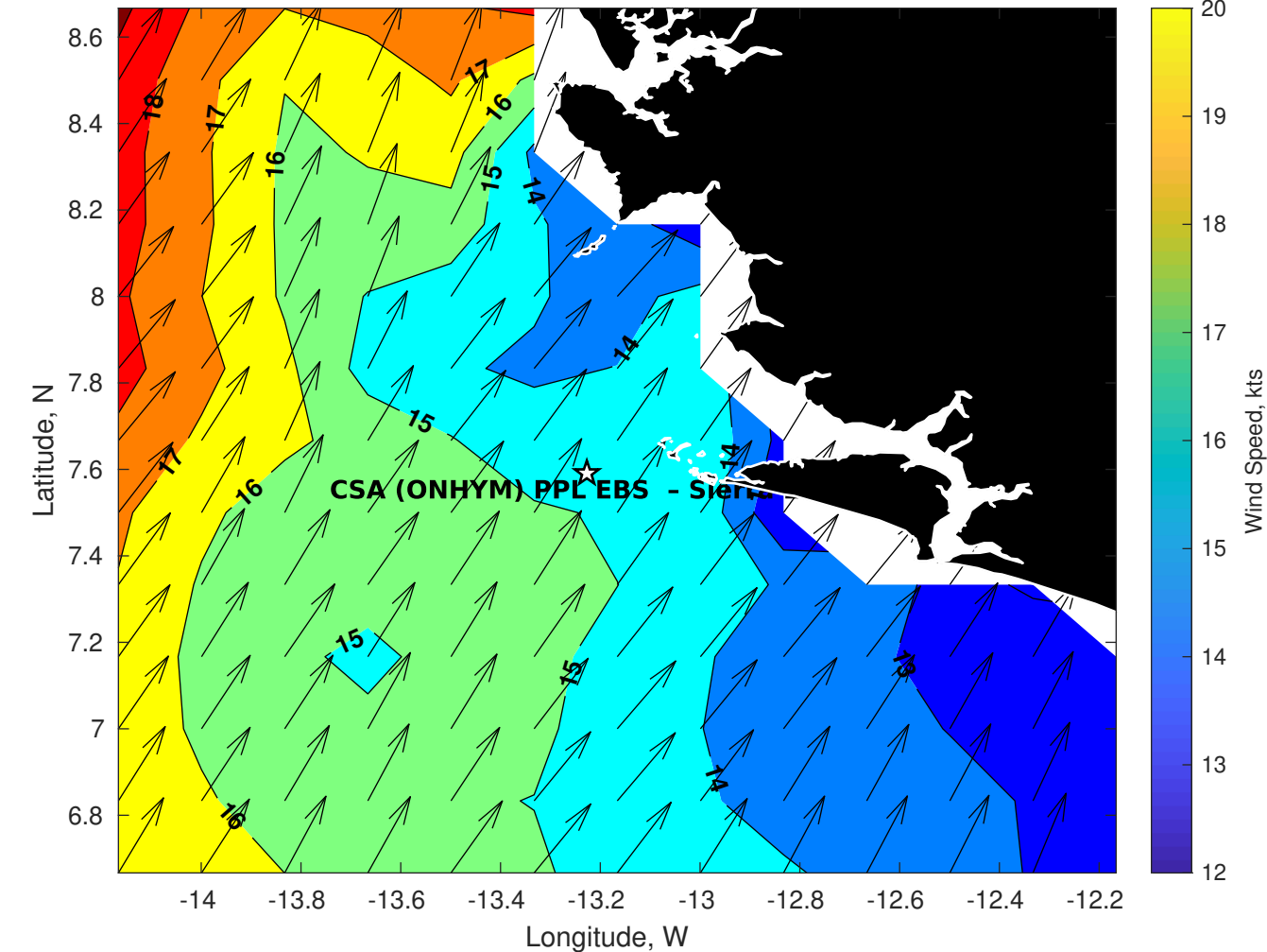
Winds (kts) for CSA (ONHYM) PPL EBS - Sierra Leone at 01-Aug-2025 09:00:00
