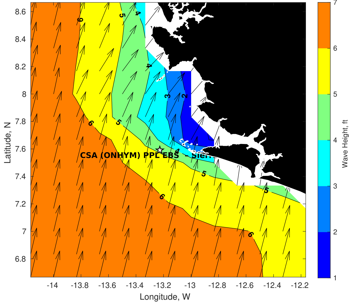
Wave Height (ft) for CSA (ONHYM) PPL EBS - Sierra Leone at 01-Aug-2025 09:00:00
