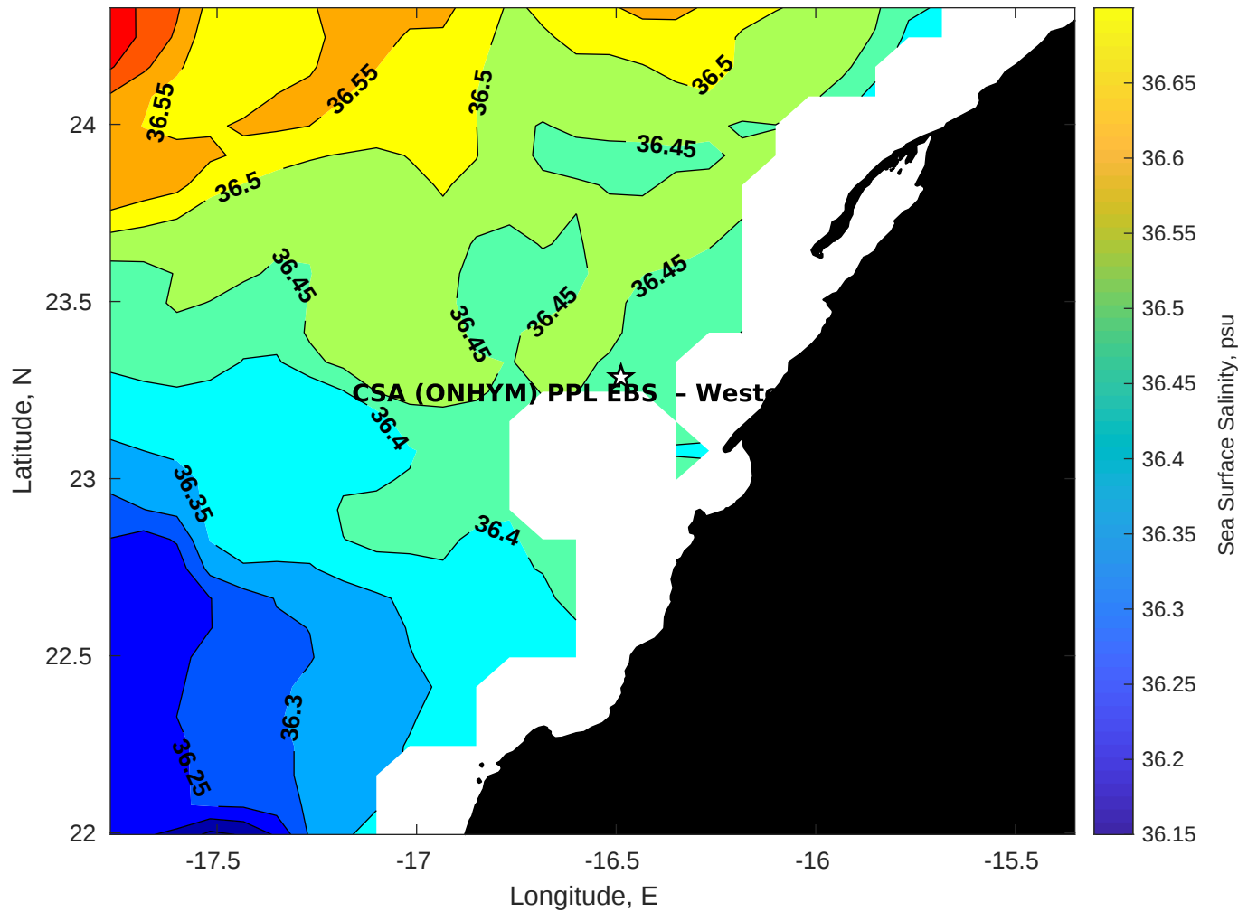
Surface Salinity for CSA (ONHYM) PPL EBS - Western Sahara at 31-Jul-2025 00:00:00
