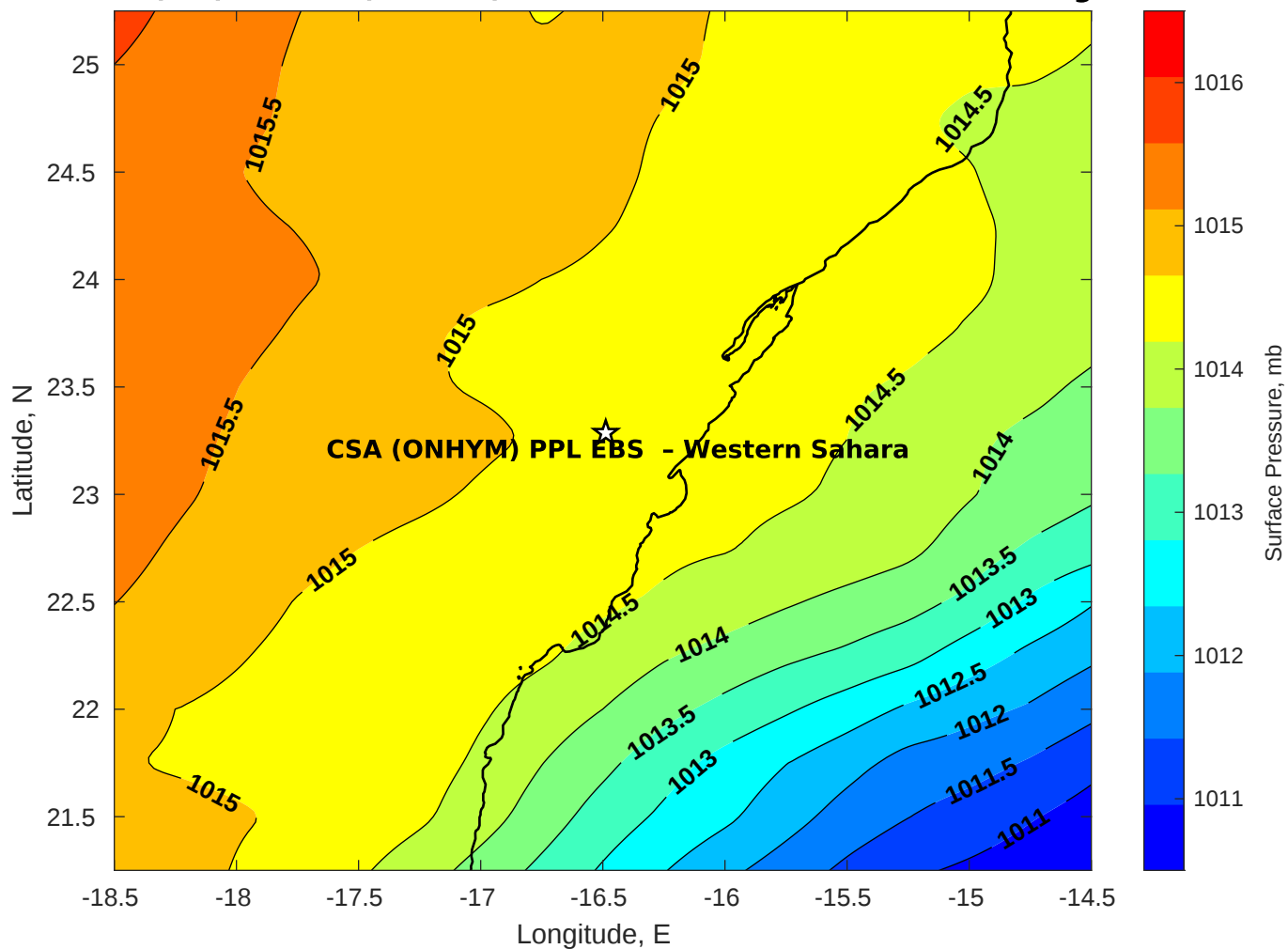
Surface Pressure (mb) for CSA (ONHYM) PPL EBS - Western Sahara at 01-Aug-2025 00:00:00
