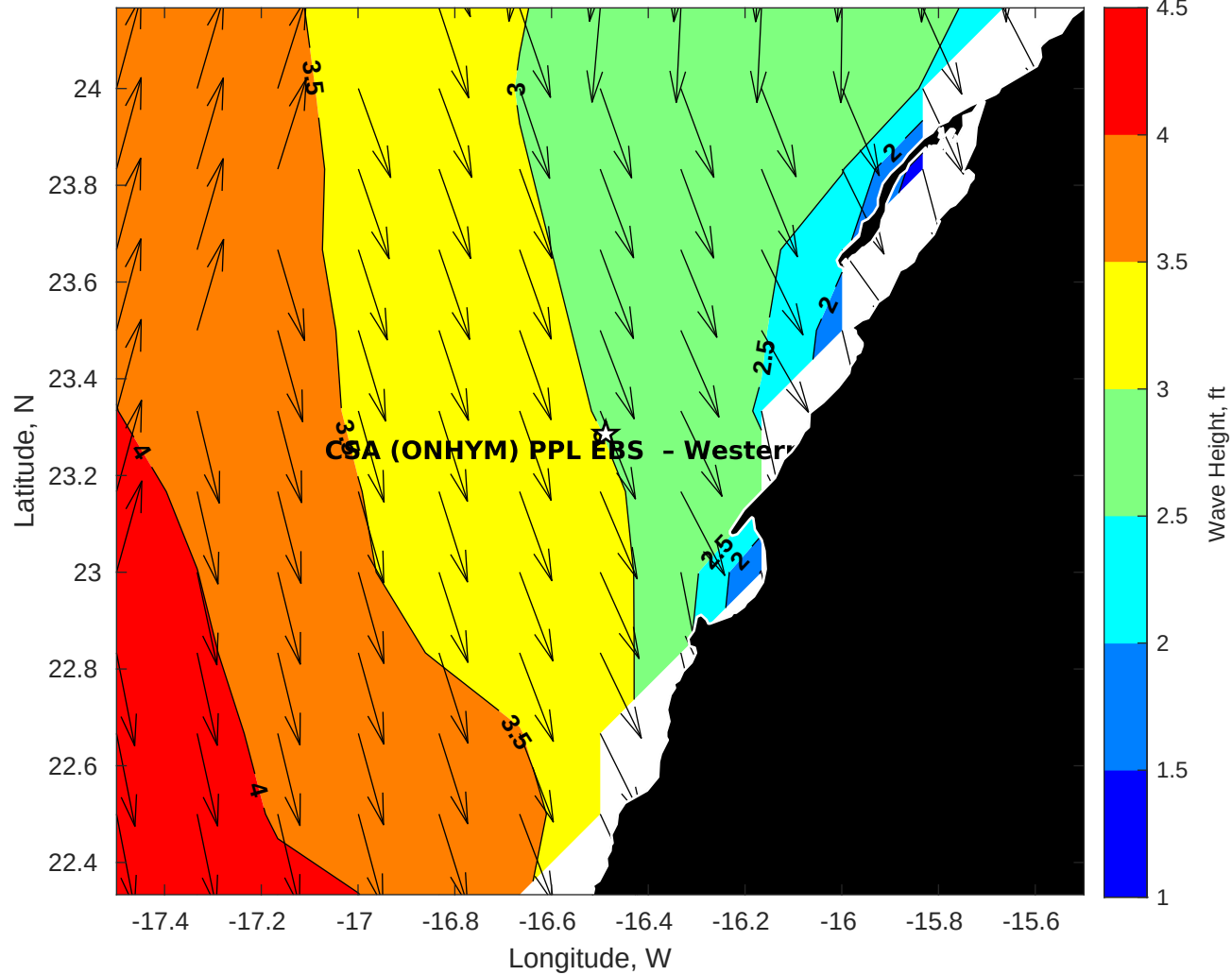
Wave Height (ft) for CSA (ONHYM) PPL EBS - Western Sahara at 01-Aug-2025 09:00:00
