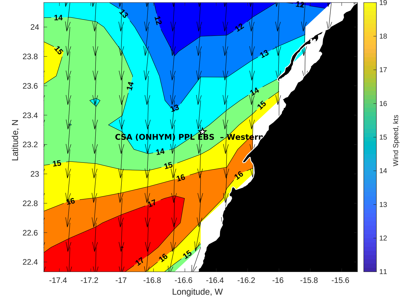
Winds (kts) for CSA (ONHYM) PPL EBS - Western Sahara at 01-Aug-2025 09:00:00
