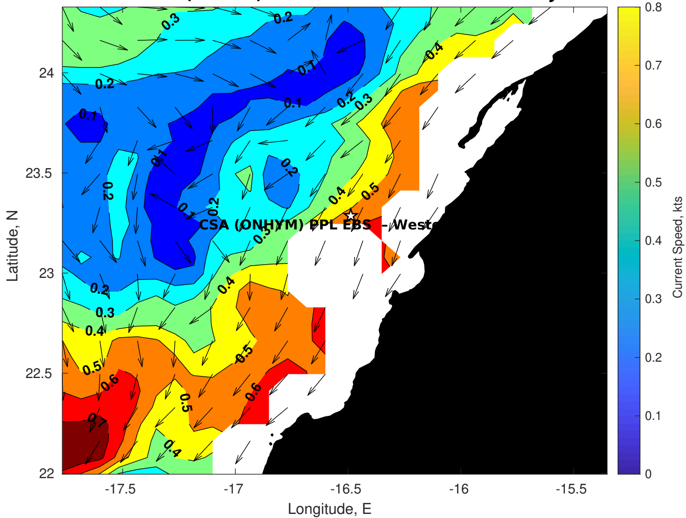
Surface Currents for CSA (ONHYM) PPL EBS - Western Sahara at 31-Jul-2025 00:00:00
