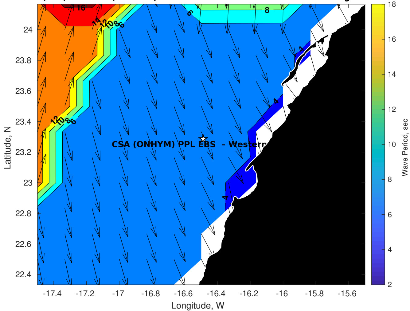
Wave Period (sec) for CSA (ONHYM) PPL EBS - Western Sahara at 01-Aug-2025 09:00:00
