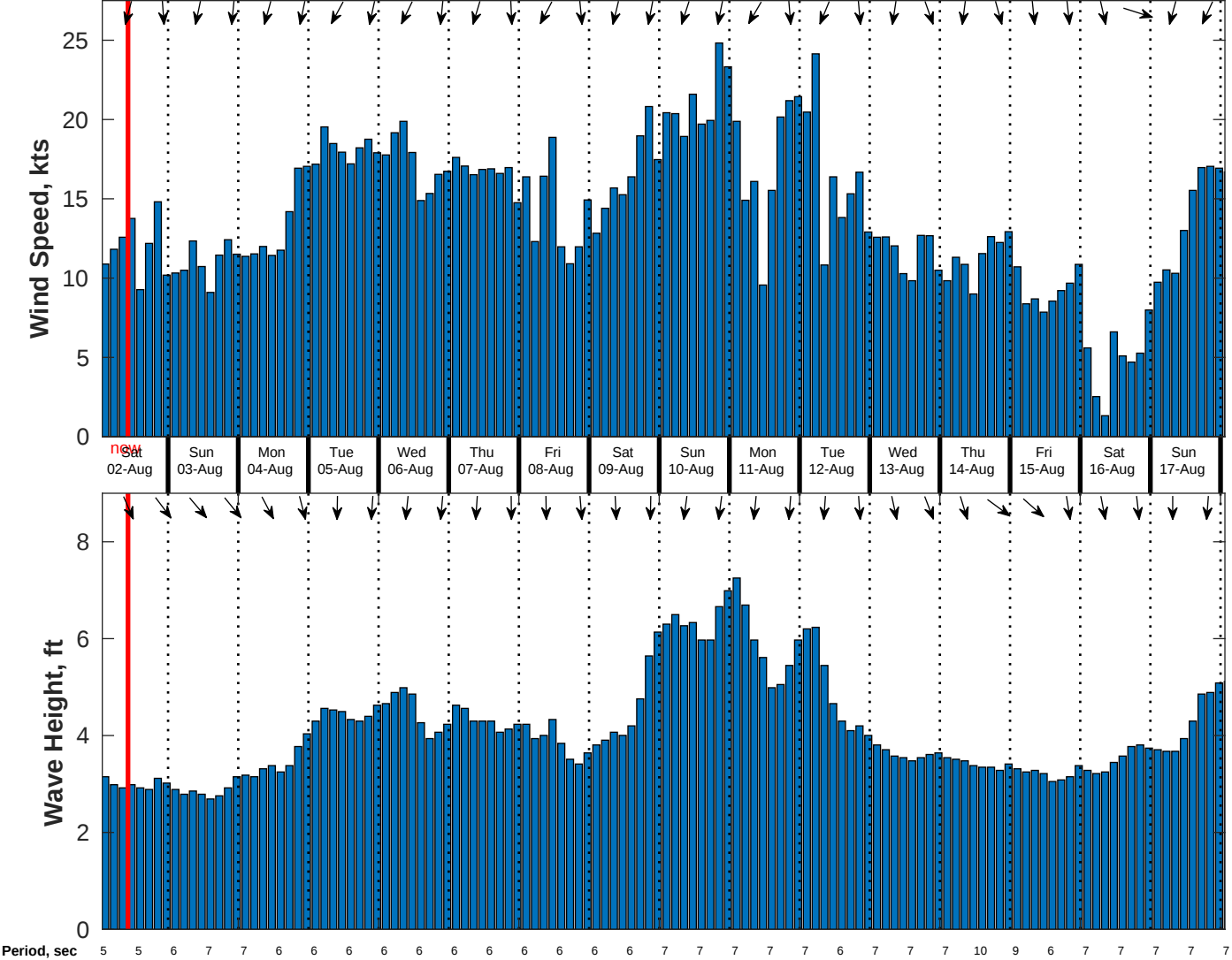
Wind & Wave Forecast for CSA (ONHYM) PPL EBS - Western Sahara from 01-Aug-2025 01:00:00 to 17-Aug-2025 01:00:00
