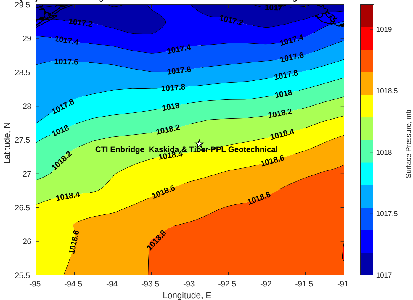
Surface Pressure (mb) for CTI Enbridge Kaskida & Tiber PPL Geotechnical at 02-Aug-2025 00:00:00
