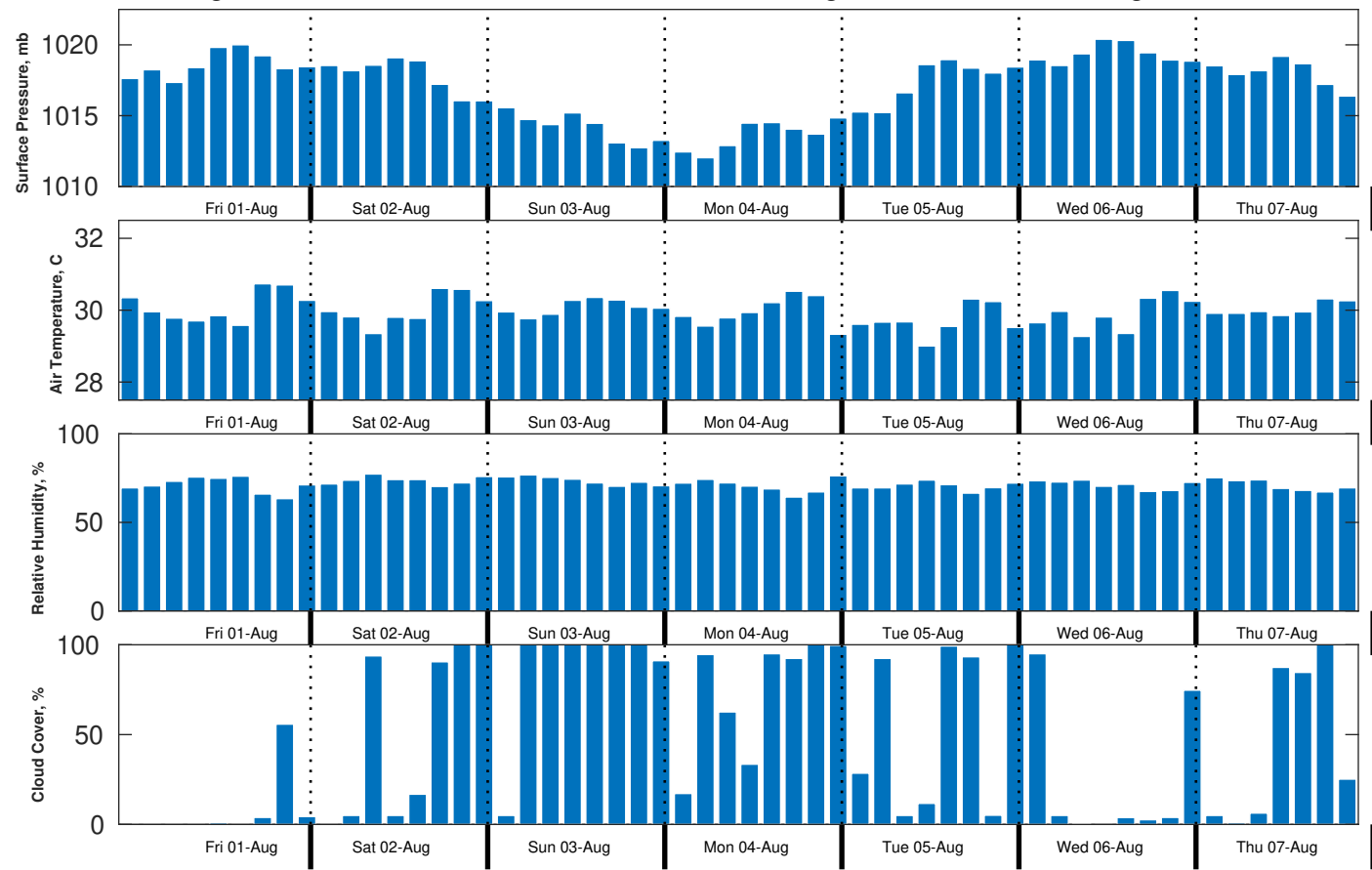
Met Forecast for CTI Enbridge Kaskida & Tiber PPL Geotechnical from 01-Aug-2025 00:00:00 to 08-Aug-2025 00:00:00
