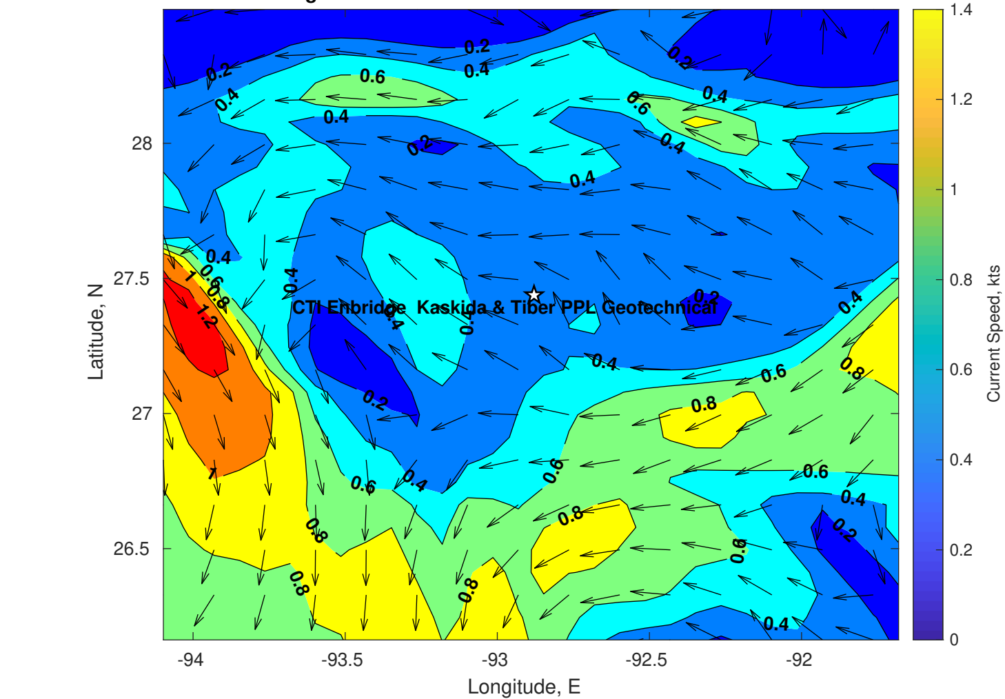
Surface Currents for CTI Enbridge Kaskida & Tiber PPL Geotechnical at 31-Jul-2025 00:00:00
