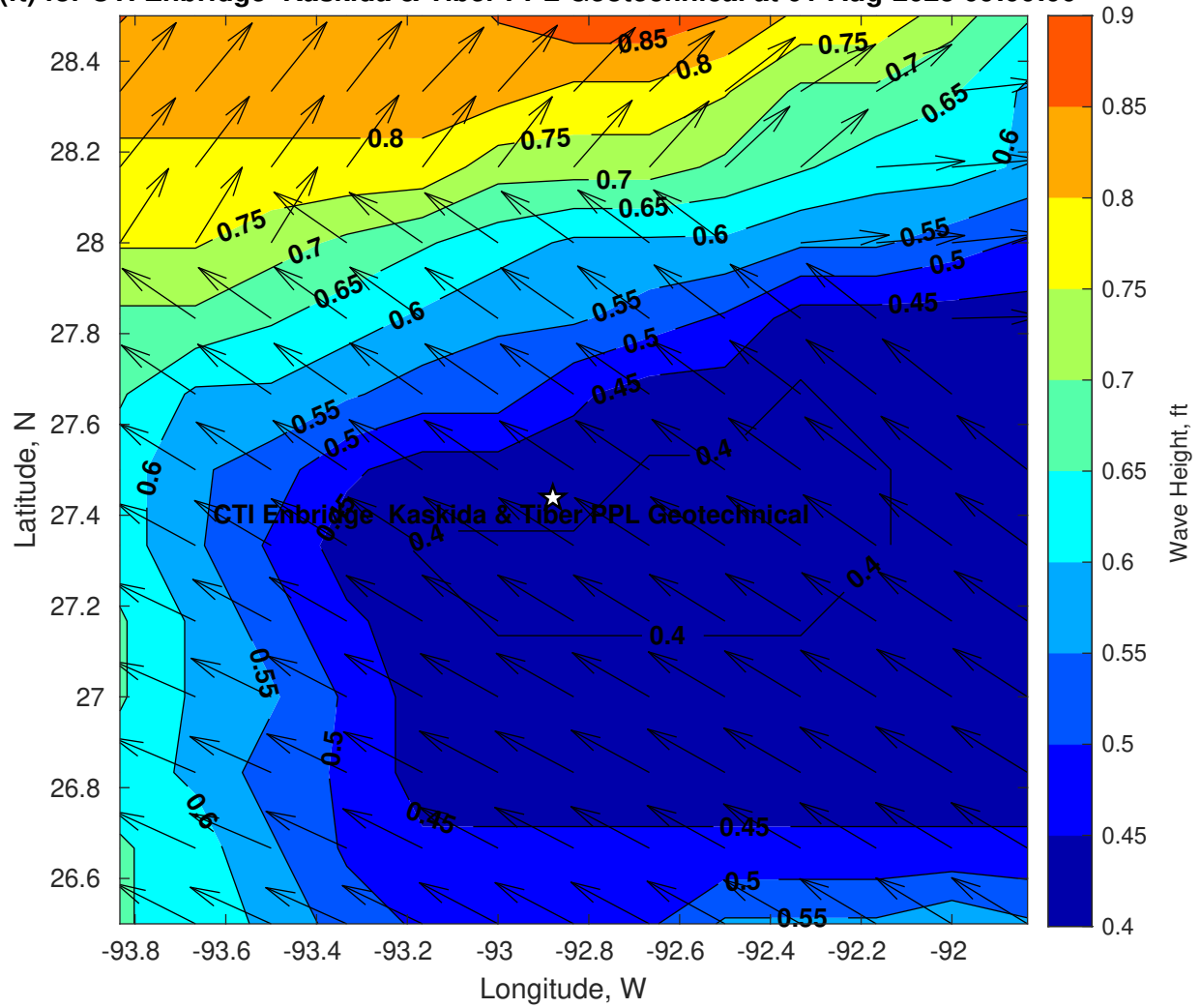
Wave Height (ft) for CTI Enbridge Kaskida & Tiber PPL Geotechnical at 01-Aug-2025 09:00:00
