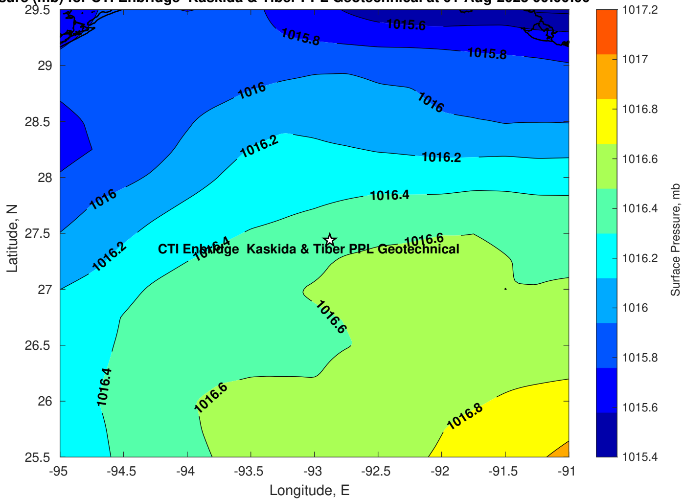
Surface Pressure (mb) for CTI Enbridge Kaskida & Tiber PPL Geotechnical at 01-Aug-2025 00:00:00
