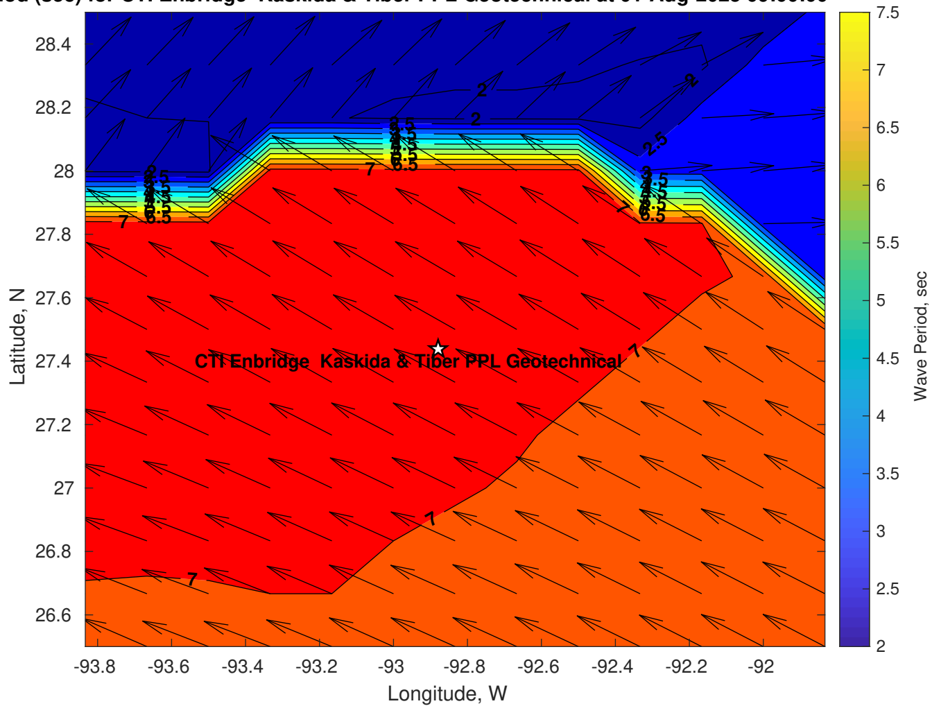
Wave Period (sec) for CTI Enbridge Kaskida & Tiber PPL Geotechnical at 01-Aug-2025 09:00:00
