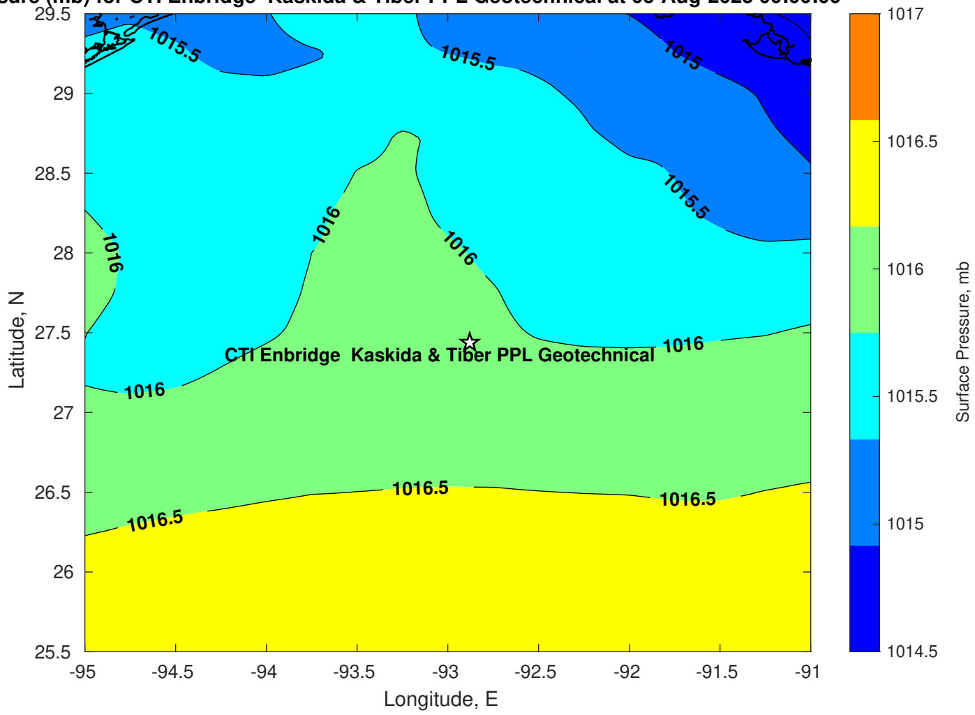
Surface Pressure (mb) for CTI Enbridge Kaskida & Tiber PPL Geotechnical at 03-Aug-2025 00:00:00
