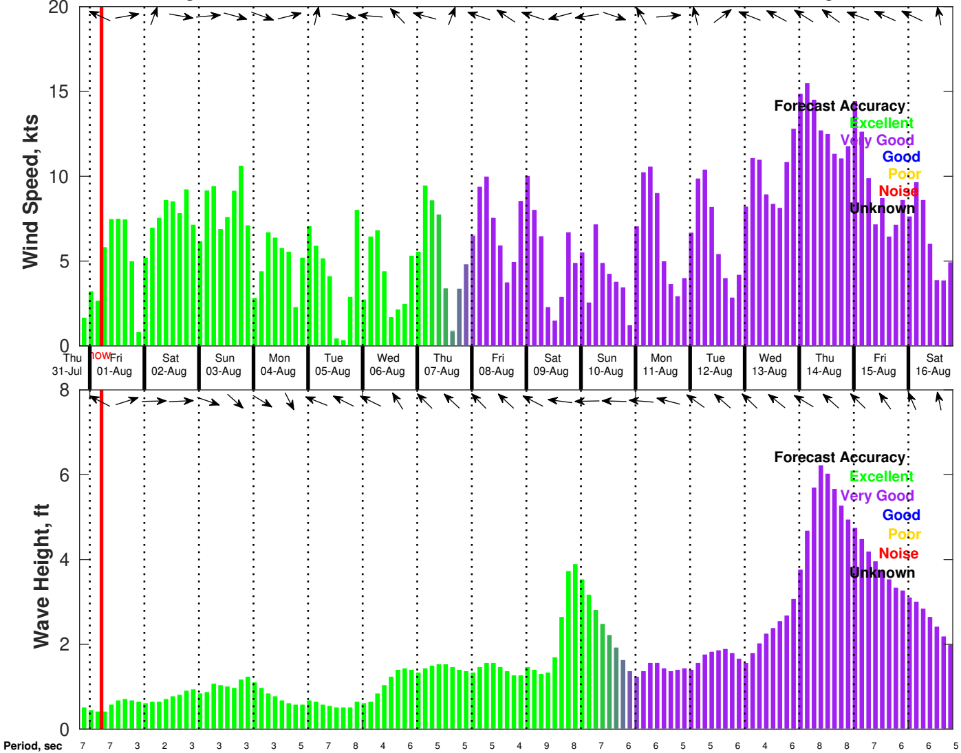
Wind & Wave Forecast for CTI Enbridge Kaskida & Tiber PPL Geotechnical from 31-Jul-2025 20:00:00 to 16-Aug-2025 20:00:00
