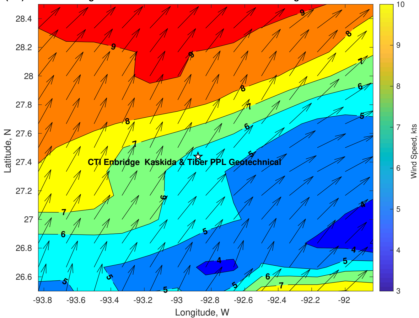
Winds (kts) for CTI Enbridge Kaskida & Tiber PPL Geotechnical at 01-Aug-2025 09:00:00
