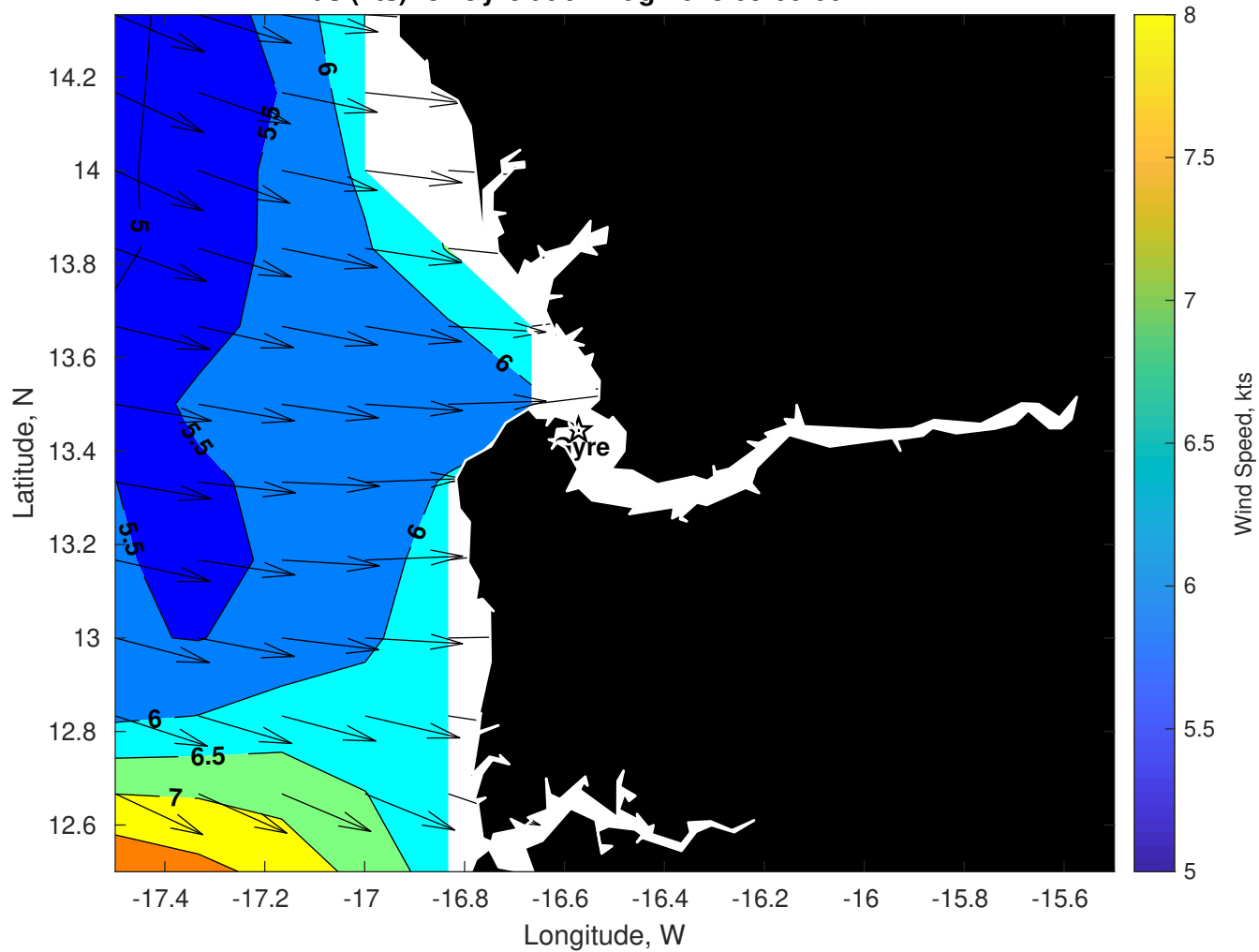
Winds (kts) for Gyre at 01-Aug-2025 09:00:00
