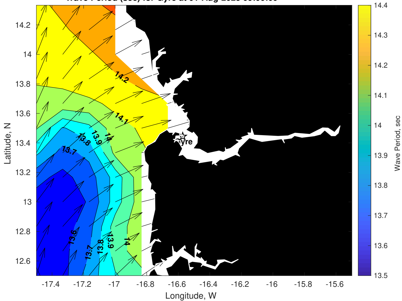
Wave Period (sec) for Gyre at 01-Aug-2025 09:00:00
