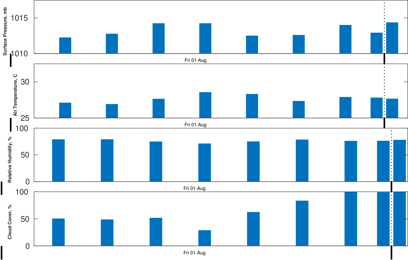
Met Forecast for Gyre from 31-Jul-2025 23:00:00 to 01-Aug-2025 22:00:00
