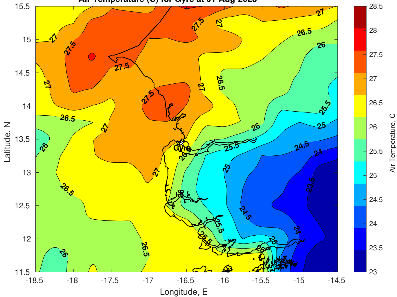
Air Temperature (C) for Gyre at 01-Aug-2025
