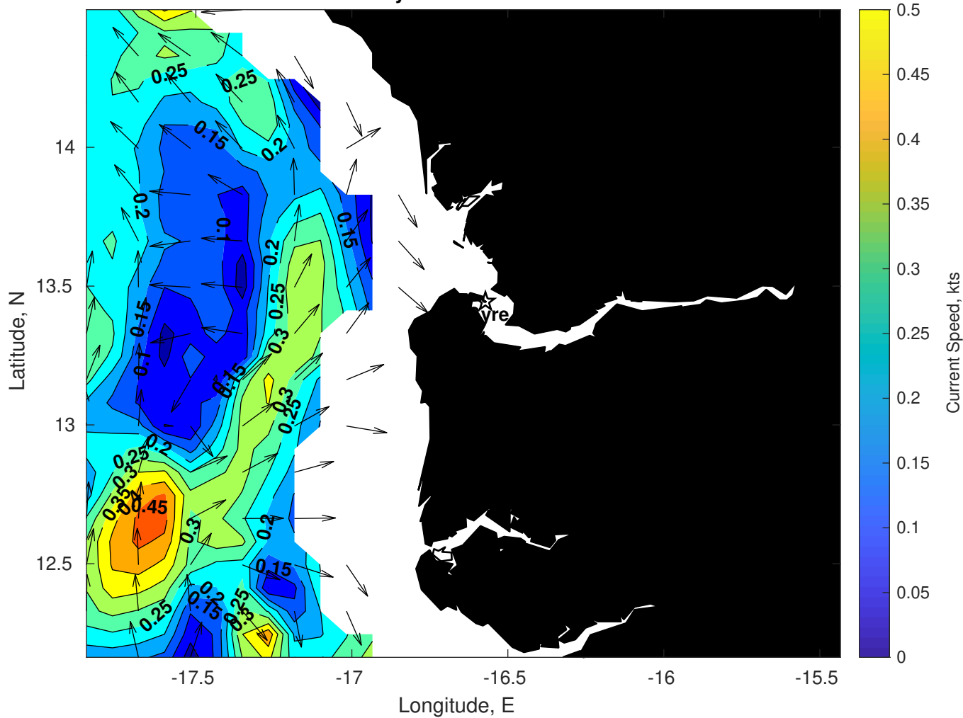
Surface Currents for Gyre at 31-Jul-2025 00:00:00
