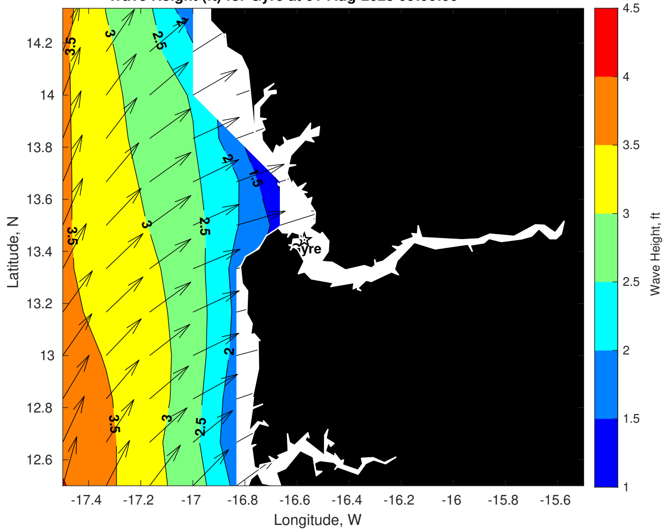
Wave Height (ft) for Gyre at 01-Aug-2025 09:00:00
