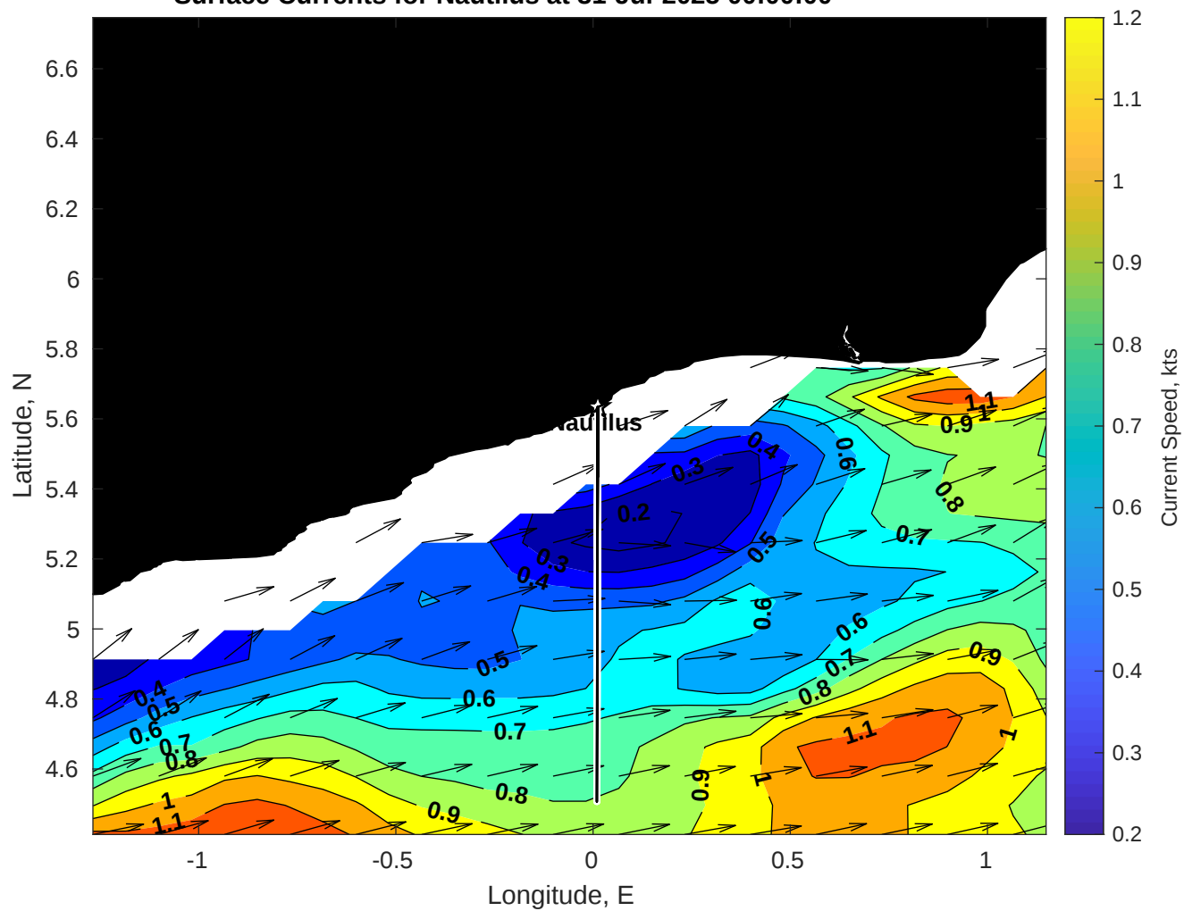
Surface Currents for Nautilus at 31-Jul-2025 00:00:00
