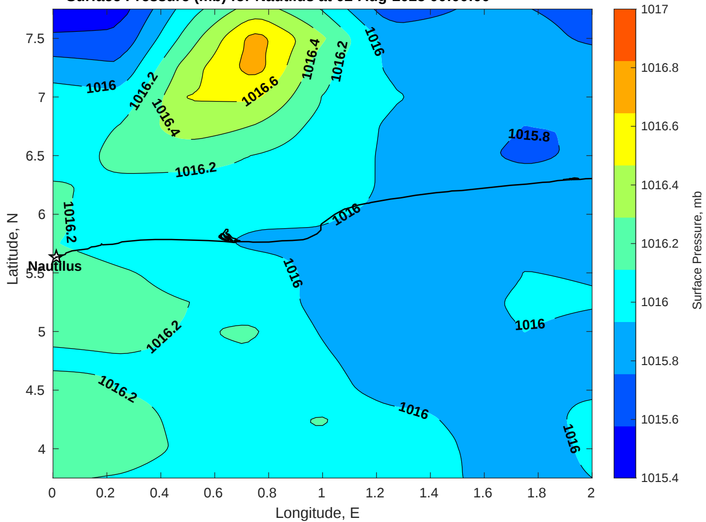
Surface Pressure (mb) for Nautilus at 02-Aug-2025 00:00:00
