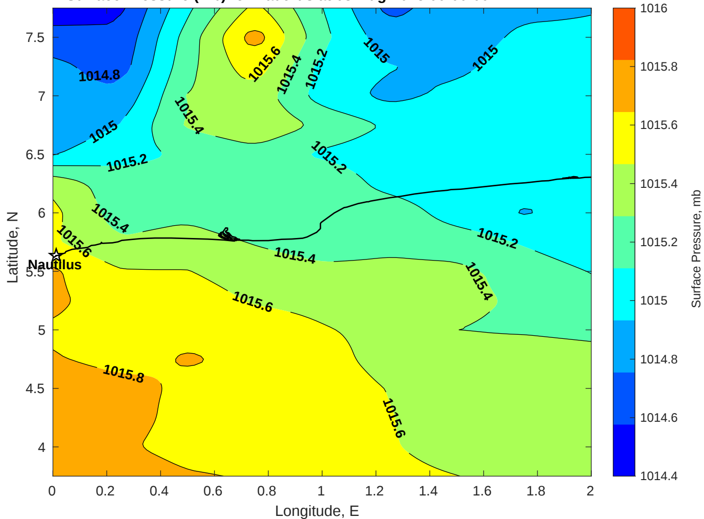
Surface Pressure (mb) for Nautilus at 03-Aug-2025 00:00:00
